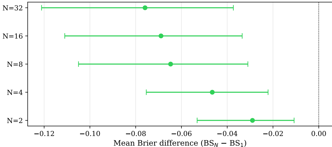
Effect sizes: Brier degradation ( w_A/w_C = 1.0 )
