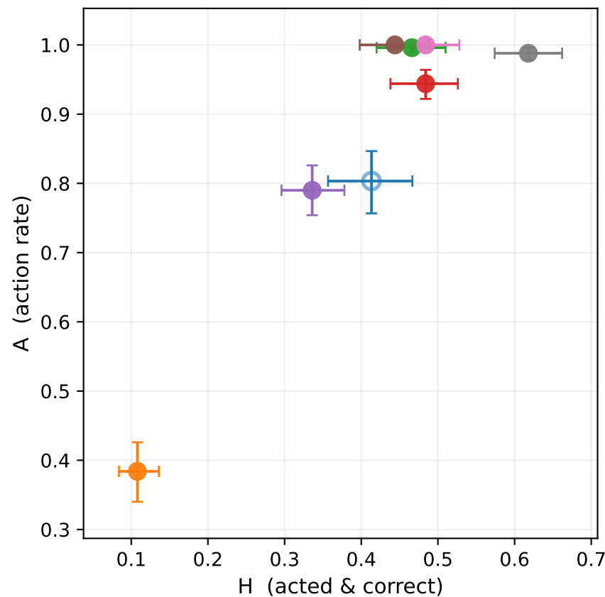
Cross-model placement of open-weights instruct models on (H, C, A)
