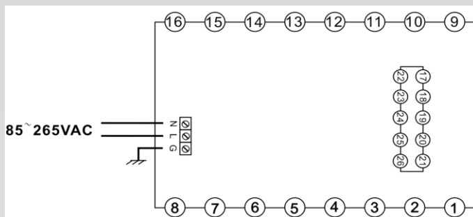
Alarm Output Diagram
