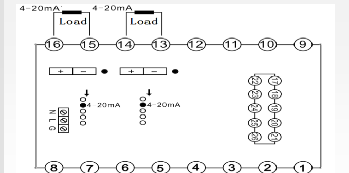
4-20mA Output Diagram
