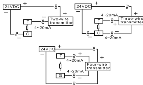
TRANSMITTER
