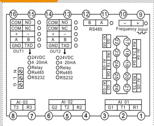
Power Diagram
