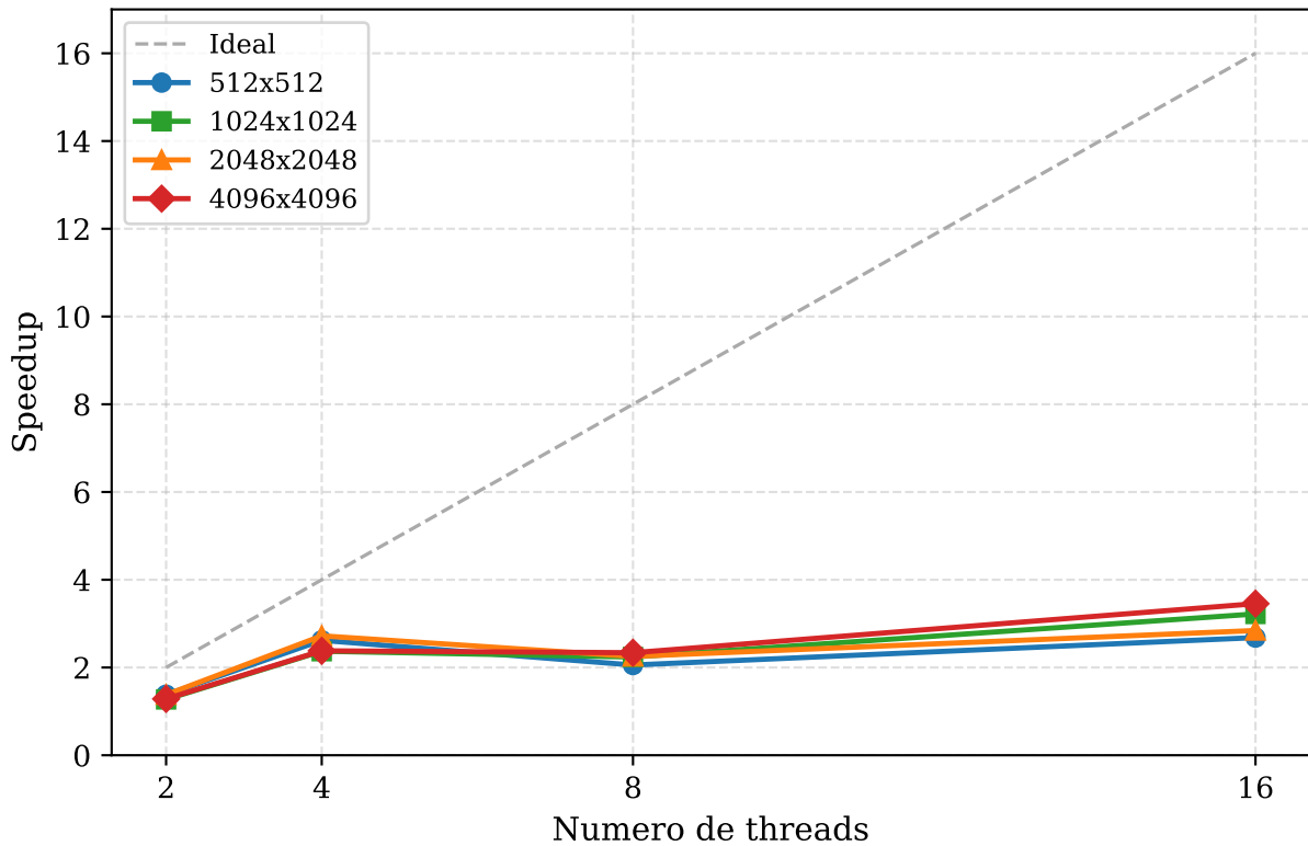
Speedup - OpenMP
