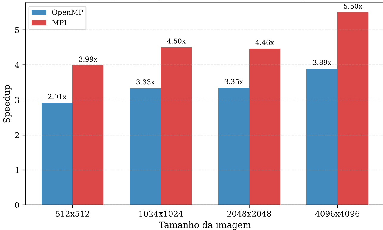
Speedup com 16 processos/threads - MPI vs OpenMP
