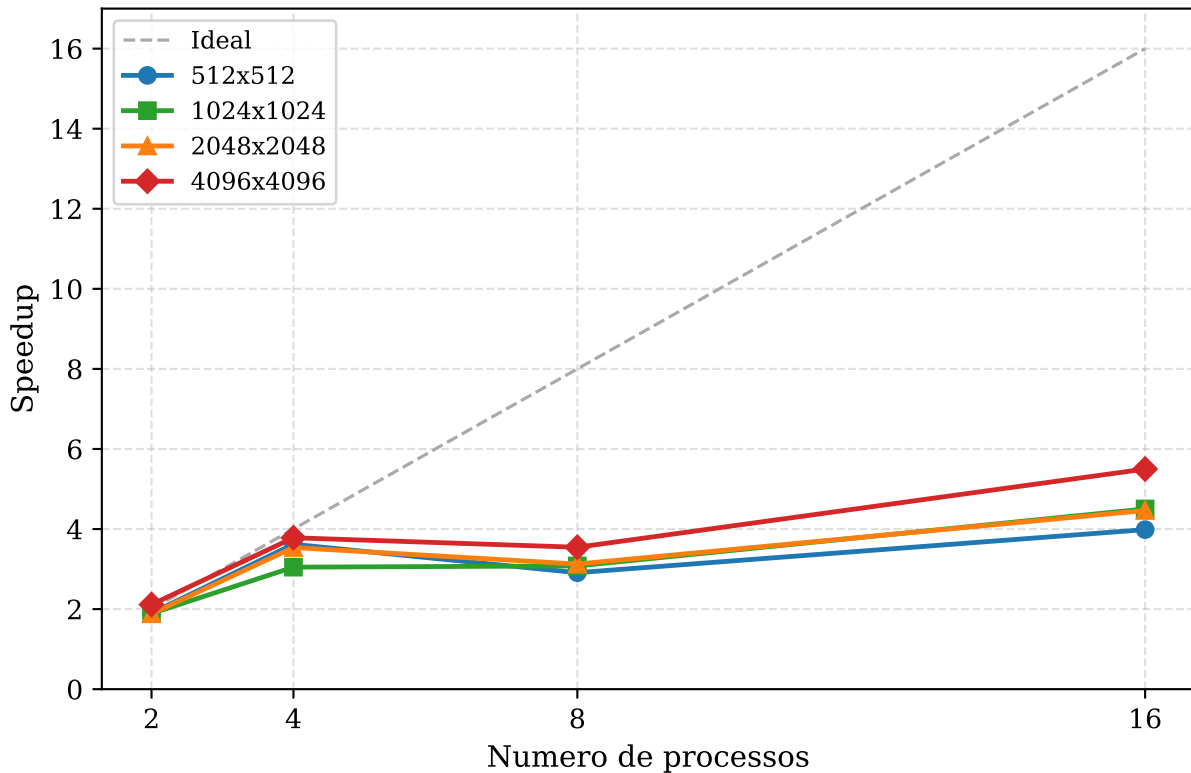
Speedup - MPI
