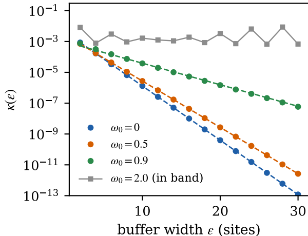
(a) sub-gap probe, \mu=3 (gap \Delta=1 )
