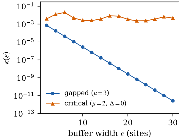
(b) same probe, gap removed
