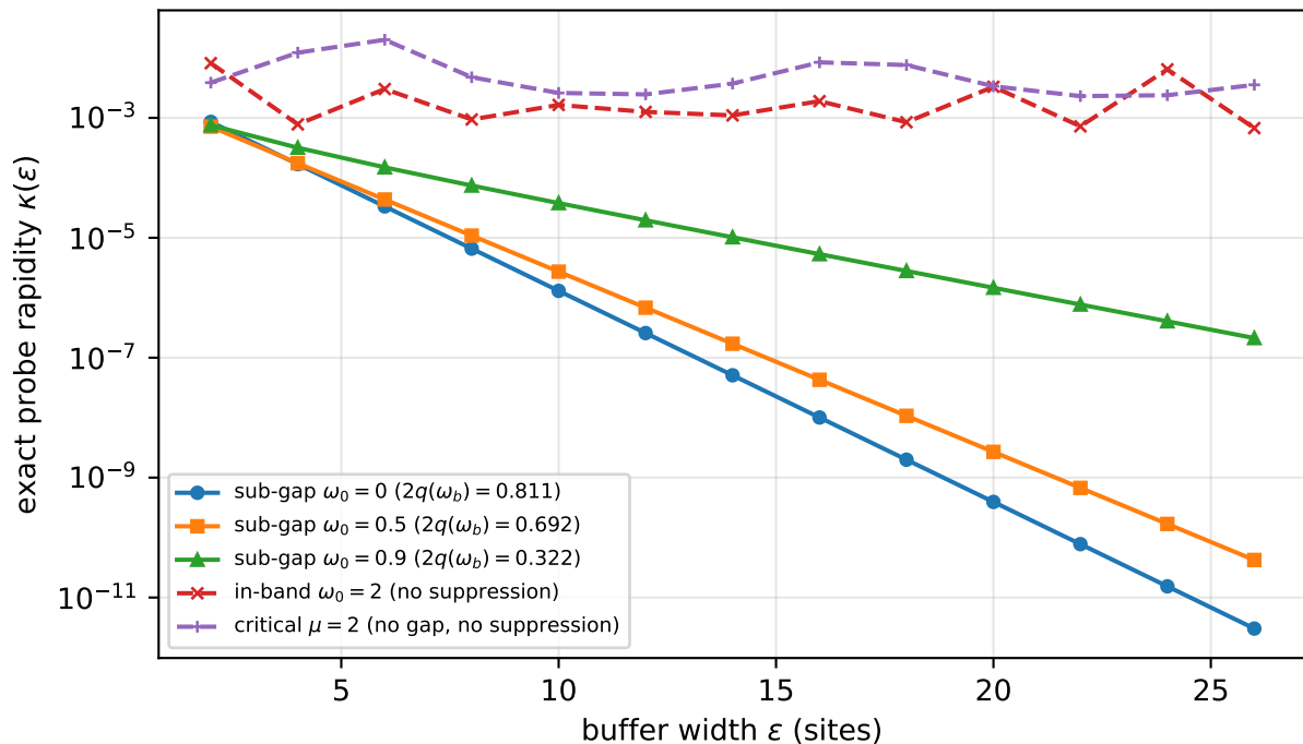
Exact rate inheritance (model of ai.viXra:2512.0064 v2) gapped buffer \mu = 3 : exponential; in-band / critical: none
