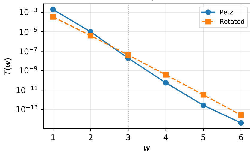
h = 1.1, \beta = 0.3
