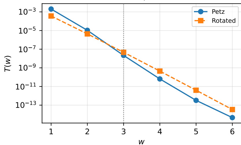
h = 1.2, \beta = 0.3
