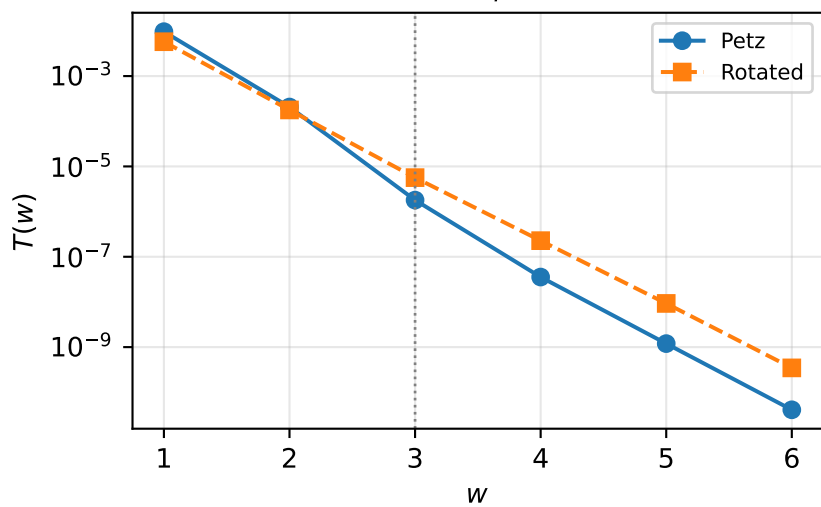
h = 1.1, \beta = 0.6
