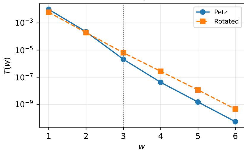
h = 1.2, \beta = 0.6
