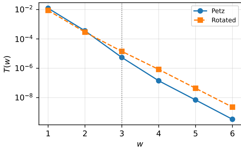
h = 1.5, \beta = 0.6
