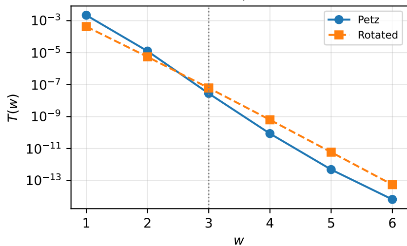
h = 1.5, \beta = 0.3
