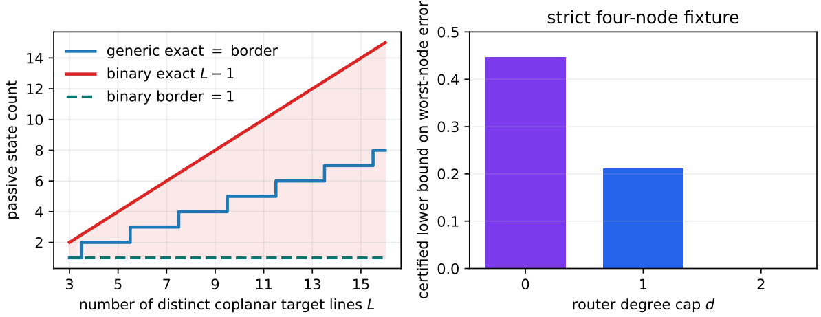
Figure 1: Left: generic exact/border memory and the binary 1 + (L - 1) split, whose exact memory is L - 1 while its border memory remains one; the shaded exact-to-border gap is unbounded. Right: exact certified worst-node chordal-error barriers for the strict four-node fixture. Degree two attains zero error, whereas degrees zero and one remain quantitatively separated.
