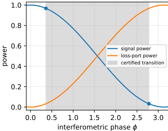
finite-error equality arc
