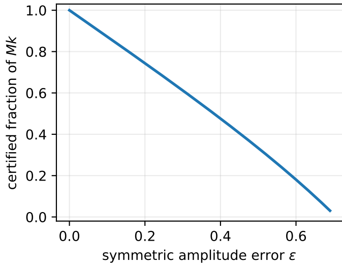
robust global degree law
