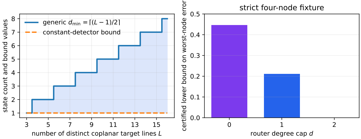
Figure 1: Left: generic exact memory versus the constant-detector lower bound; the multiplicative ratio is unbounded. Right: exact certified worst-node chordal-error barriers for the strict four-node fixture. Degree two attains zero error, whereas degrees zero and one remain quantitatively separated.
