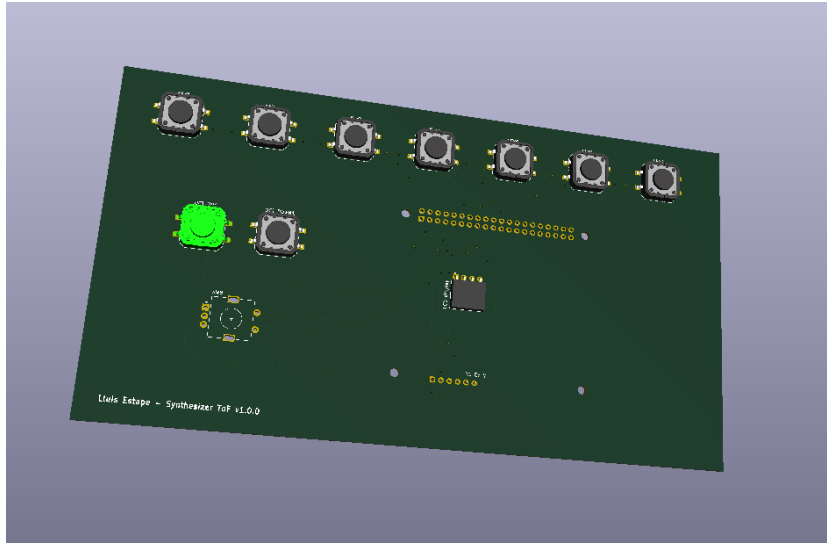
Figure 8: LaserHarp: 3D render of the ToF synthesizer PCB (v1.0.0).
