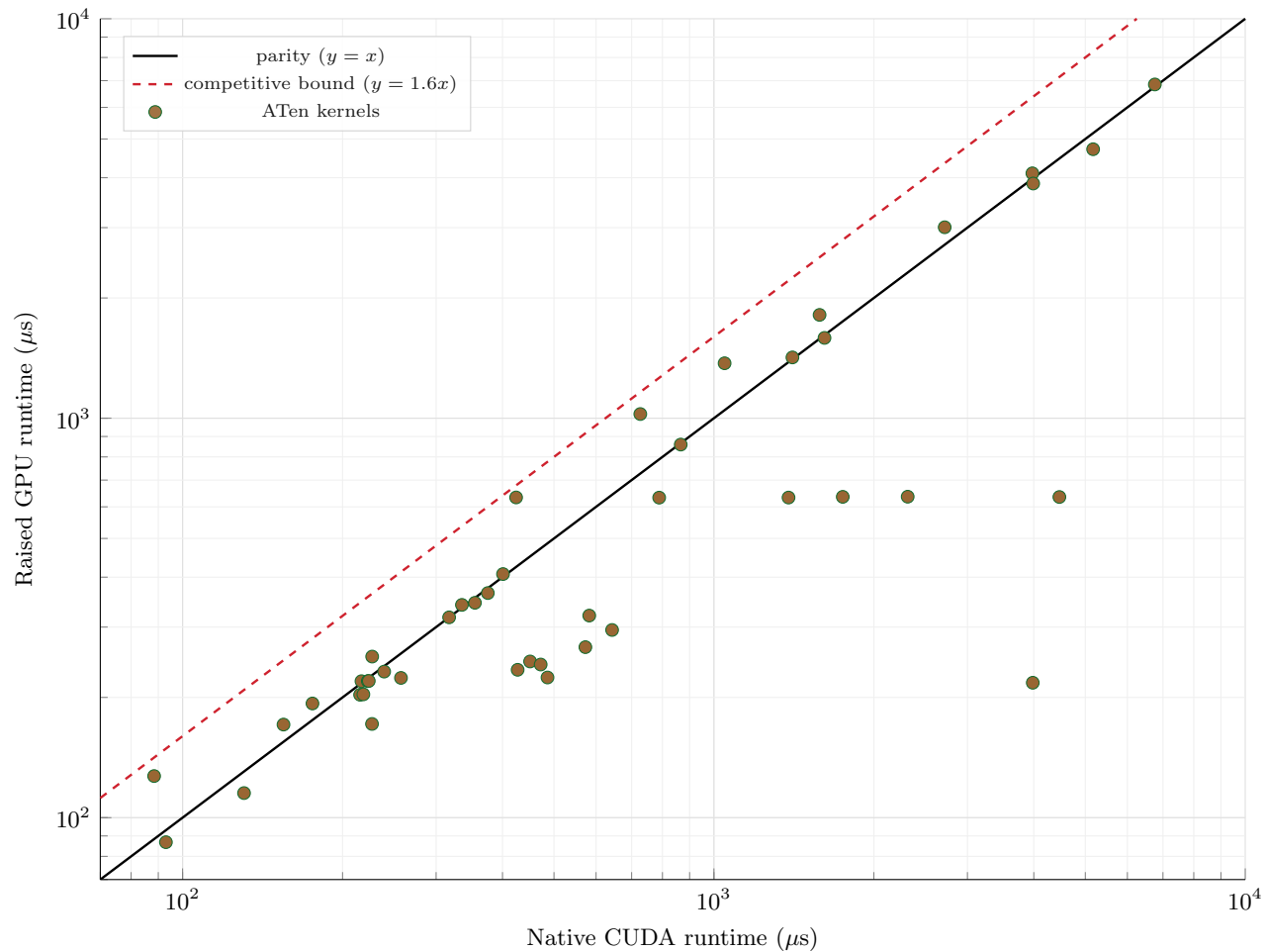
ATen: raised GPU vs native GPU runtime
