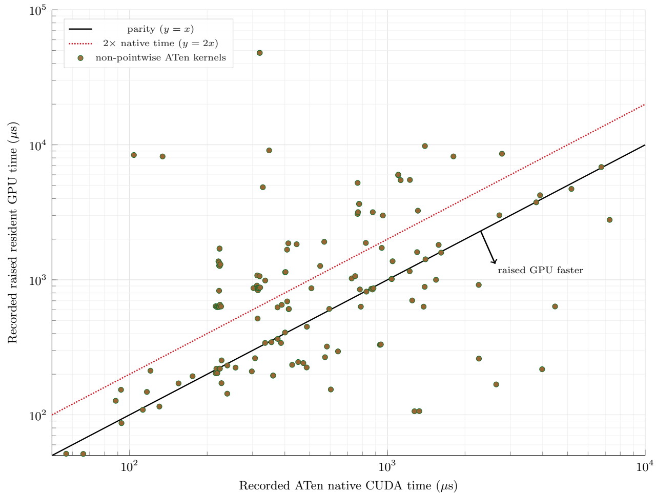
ATen: 142 non-pointwise raised vs native GPU runtimes
