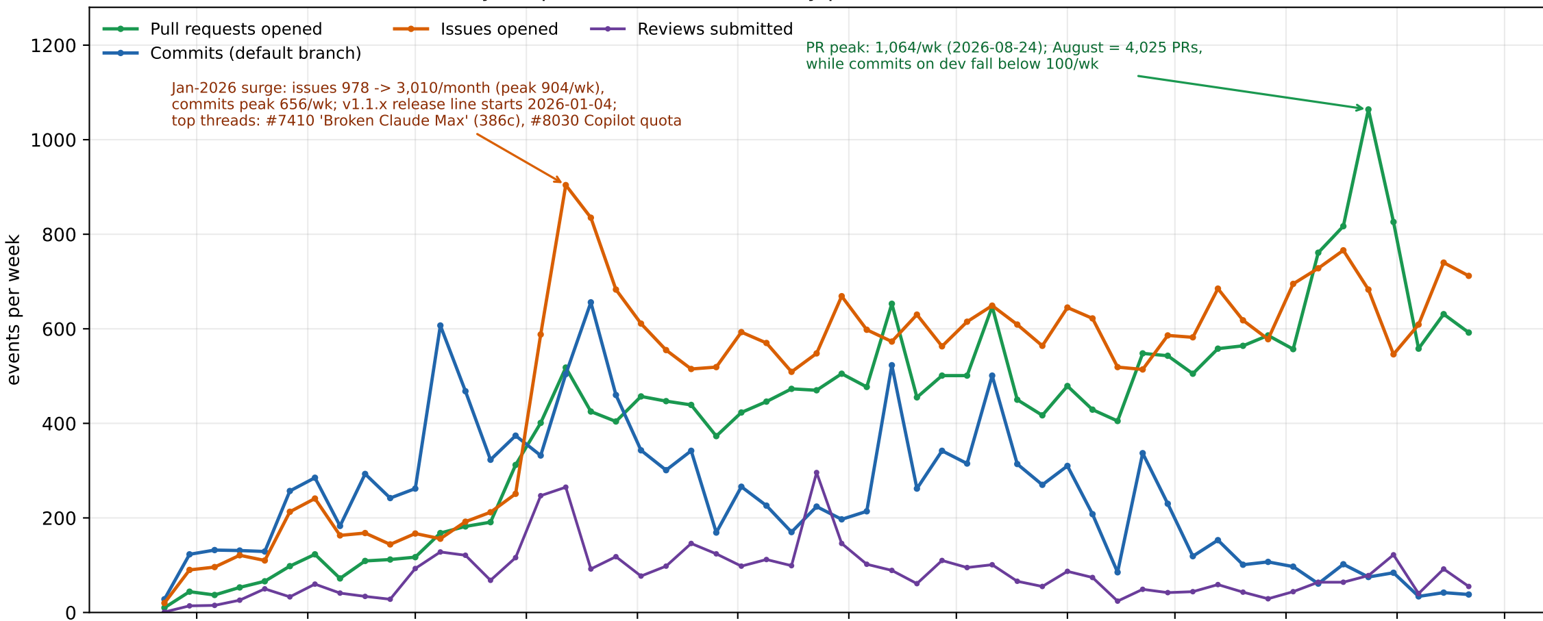
anomalyco/opencode - GitHub activity per week, 2025-09-27 to 2026-09-27
