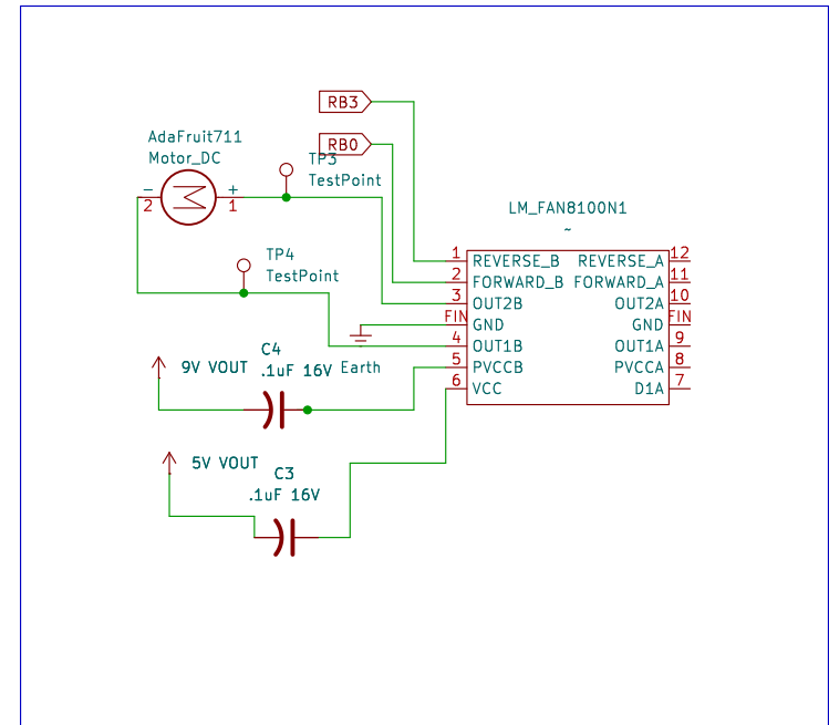
H-BRIDGE AND DC MOTOR
