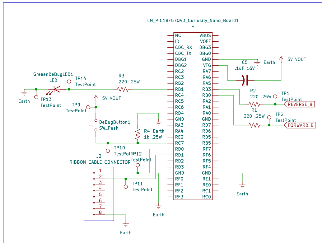
MICROCONTROLLER AND RIBBON CABLE CONNECTOR
