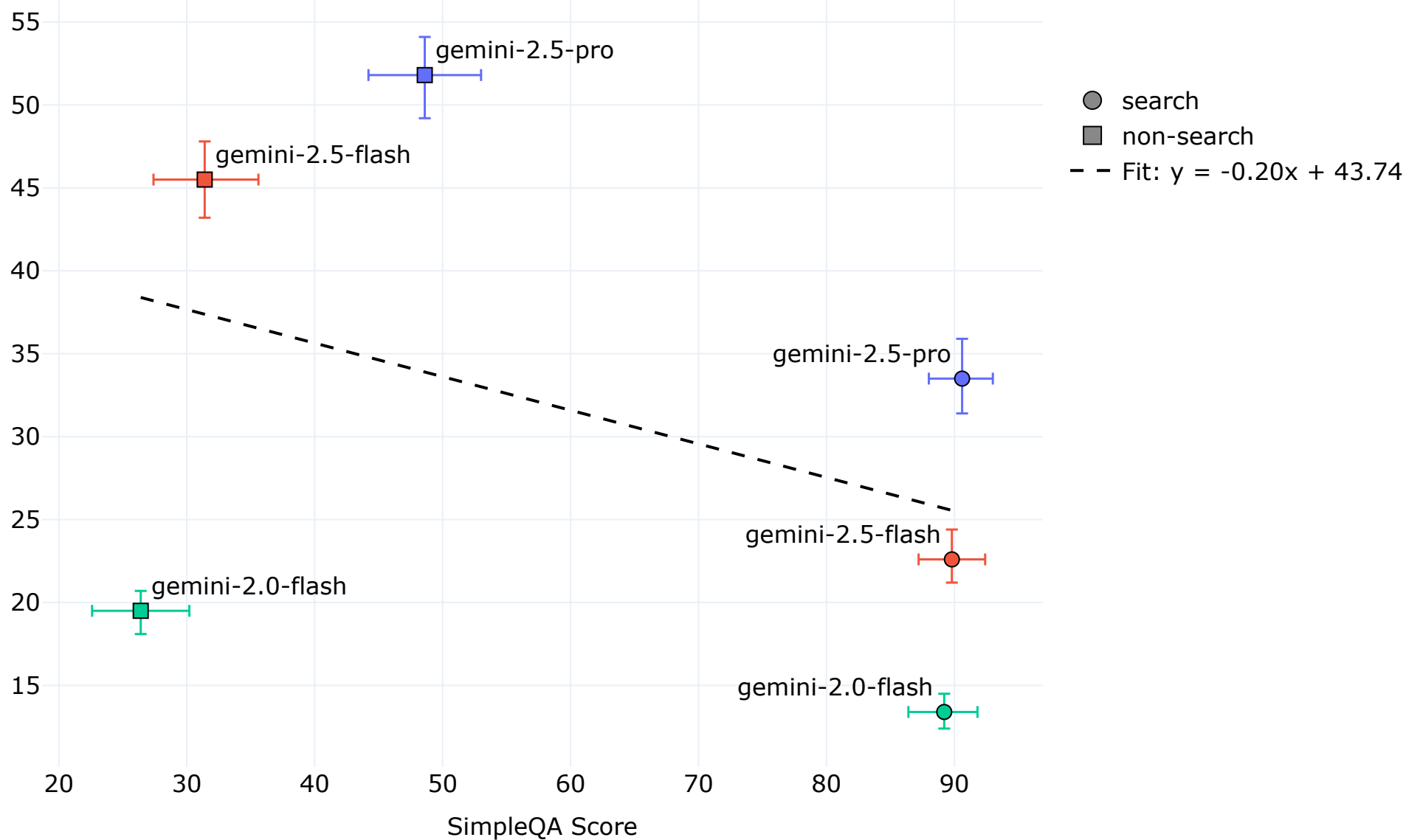
ArenaHard Score
