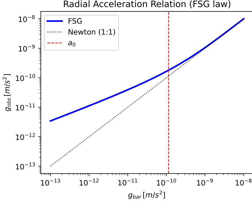
Figure 6: Radial Acceleration Relation (RAR): the FSG prediction is identical to the empirical relation, with transition at g_{\text{bar}} = a_0 .
