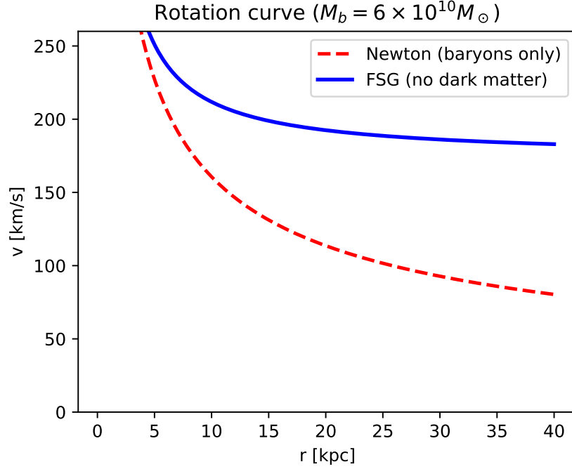
Figure 4: Newtonian potential ( 1/r ) decays rapidly, producing v \propto r^{-1/2} . FSG's fractal potential ( \ln r ) leads to v = \text{const.}
