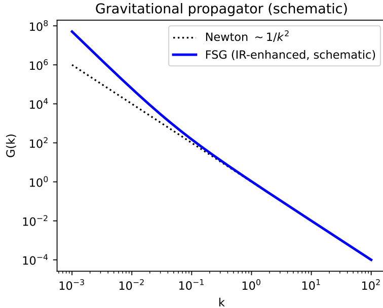
Figure 2: Comparison of the Newtonian propagator 1/k^2 with the FSG infrared propagator 1/k^3 (required for MOND dynamics).
