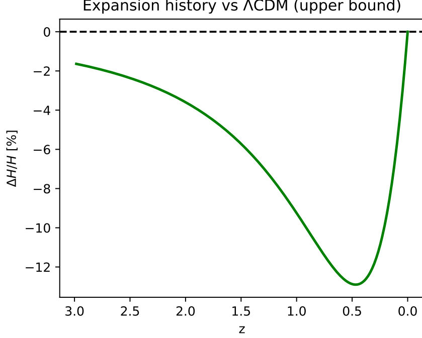
Figure 11: Relative deviation of H(z) between FSG and \Lambda CDM. Euclid will detect differences > 1\% .
