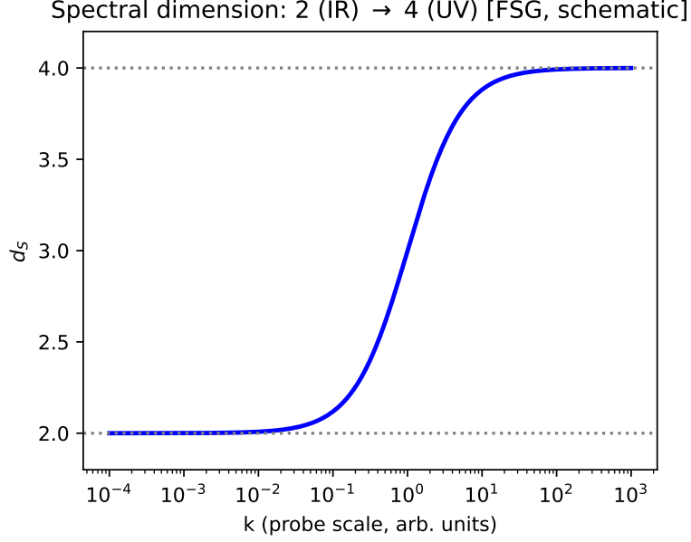
Figure 1: Illustrative running of the spectral dimension as a function of energy scale. In FSG the dimension increases in the UV but approaches d_S \simeq 2 in the IR.
