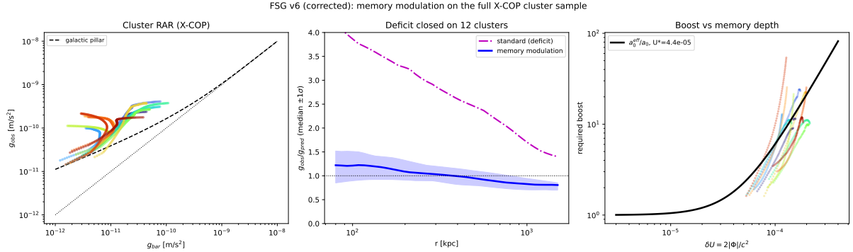
Figure 8: Cluster mass budget on the 12 X-COP clusters ( simulations/sim_xcop_clusters.py ). Left: cluster RAR, lying above the galactic relation. Middle: the median deficit g_{\text{obs}}/g_{\text{pred}} (dot-dashed, factor \sim 3 ) closed by memory modulation (solid, unity) with a single U_{\star} . Right: the required boost versus memory depth \delta U , against a_0^{\text{eff}} = a_0[1 + (\delta U/U_{\star})^2] .
