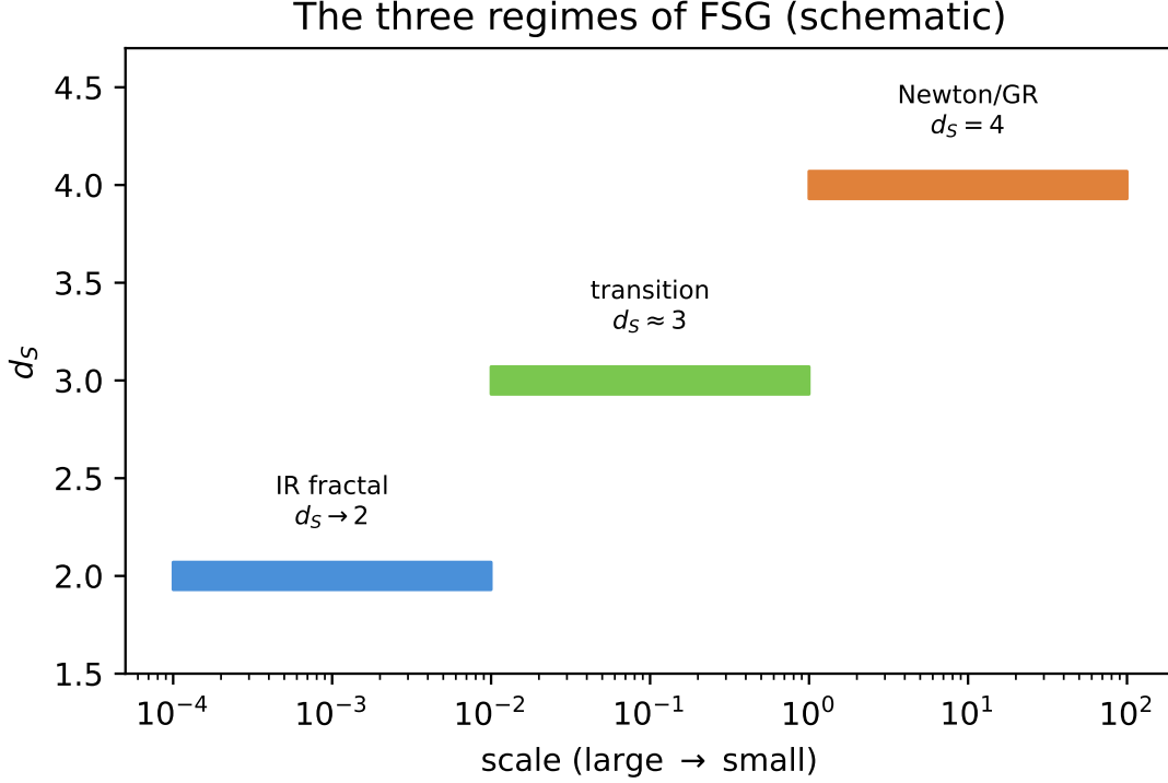
Figure 13: Schematic summary of the three regimes of FSG: (1) Newton/GR regime ( d_S = 4 ), (2) transition regime ( d_S \approx 3 ), (3) fractal IR regime ( d_S \rightarrow 2 ).
