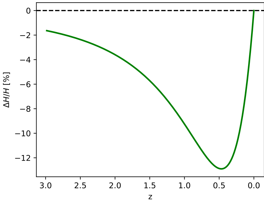
Expansion history vs \Lambda CDM (upper bound)
