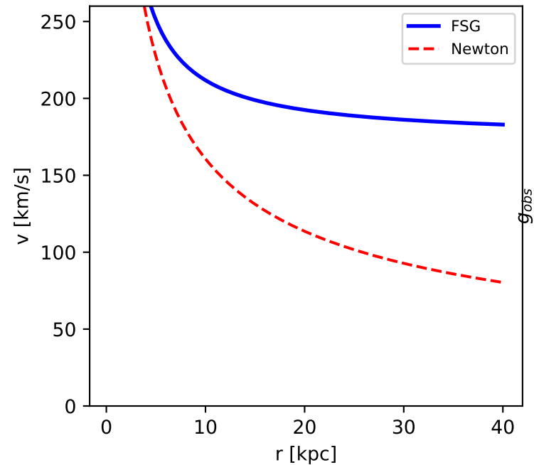
A. Flat rotation curve
