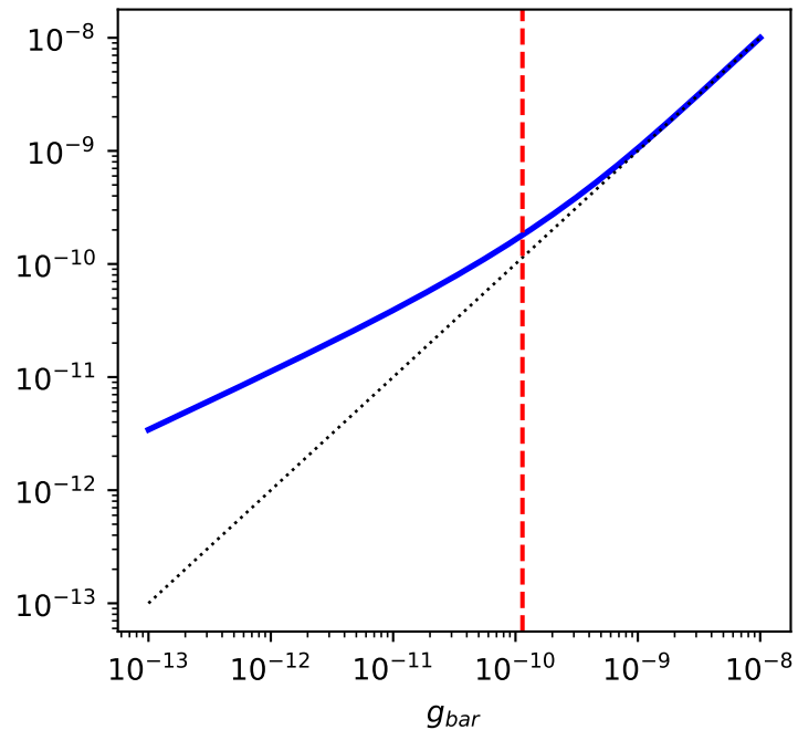
B. Radial acceleration relation
