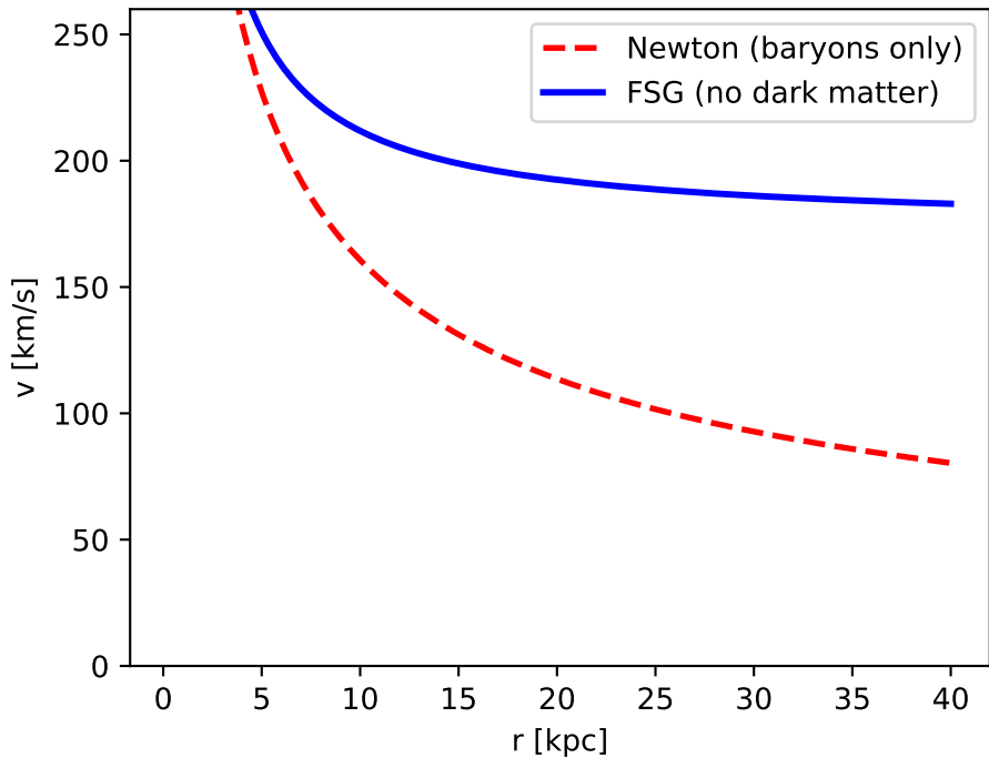
Rotation curve ( M_b = 6 \times 10^{10} M_\odot )
