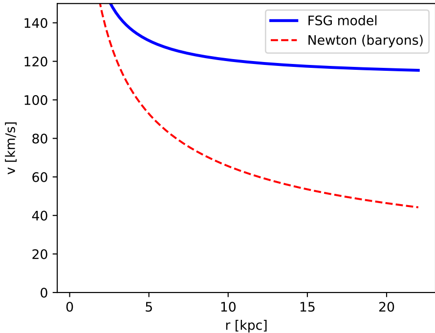
NGC 6503-mass FSG model ( M_b \sim 10^{10} M_\odot ; not a fit)
