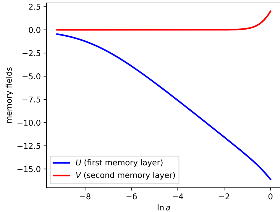
Cosmic memory build-up
