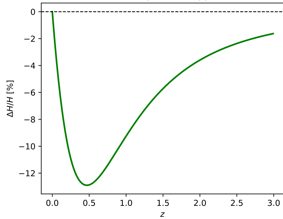
FSG vs LCDM expansion (upper bound)
