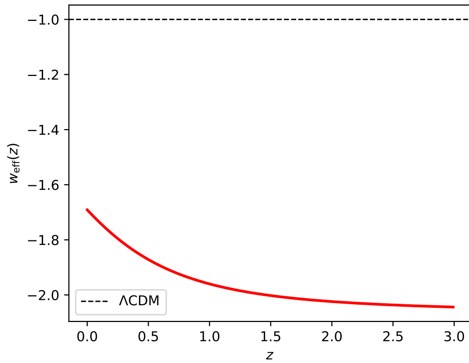
Effective EoS, upper bound ( w_0 = -1.69 )
