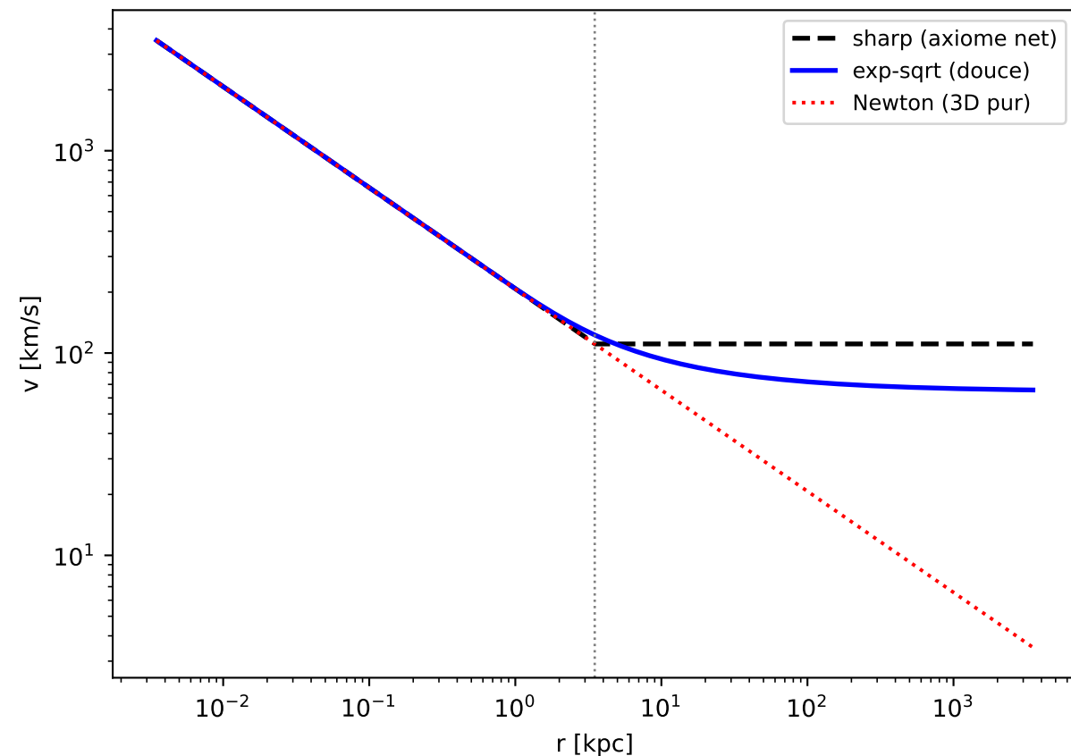
Diversite : transition a r_M = \sqrt{GM/a_0} (pointilles)
