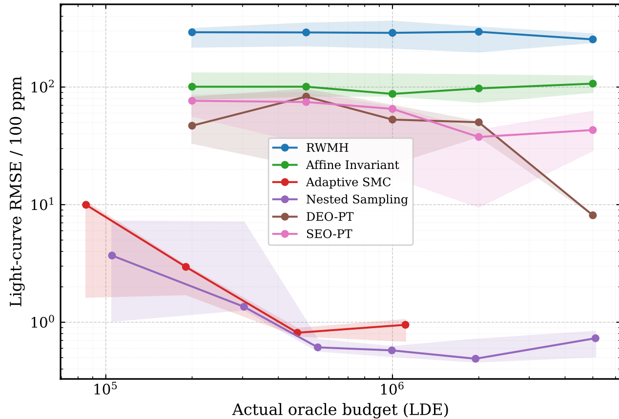
Best-fit light-curve RMSE vs. actual oracle budget
