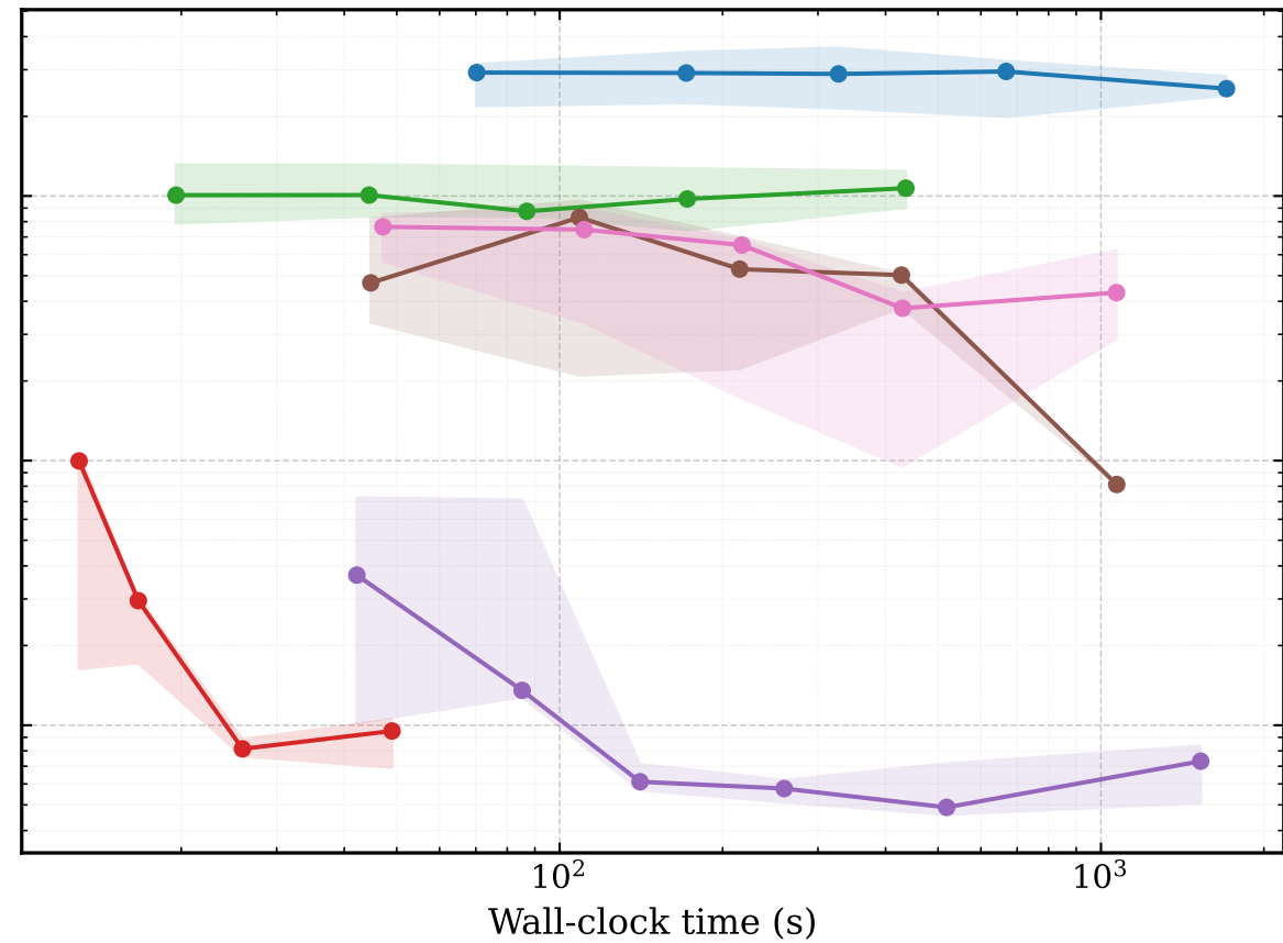
Best-fit light-curve RMSE vs. wall-clock time
