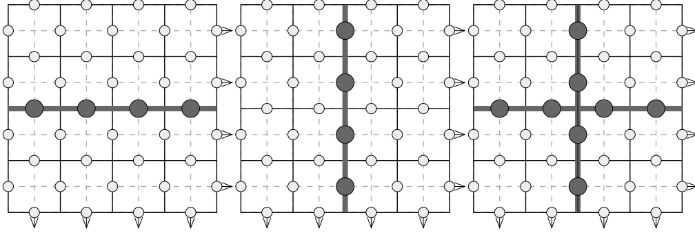
Fig. 4: Three of the four independent degenerate ground state groups. The fourth is the empty lattice.
