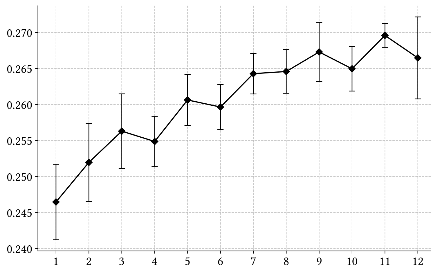
Point-BERT
