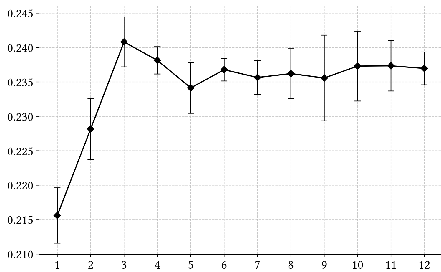
Point-MAE
