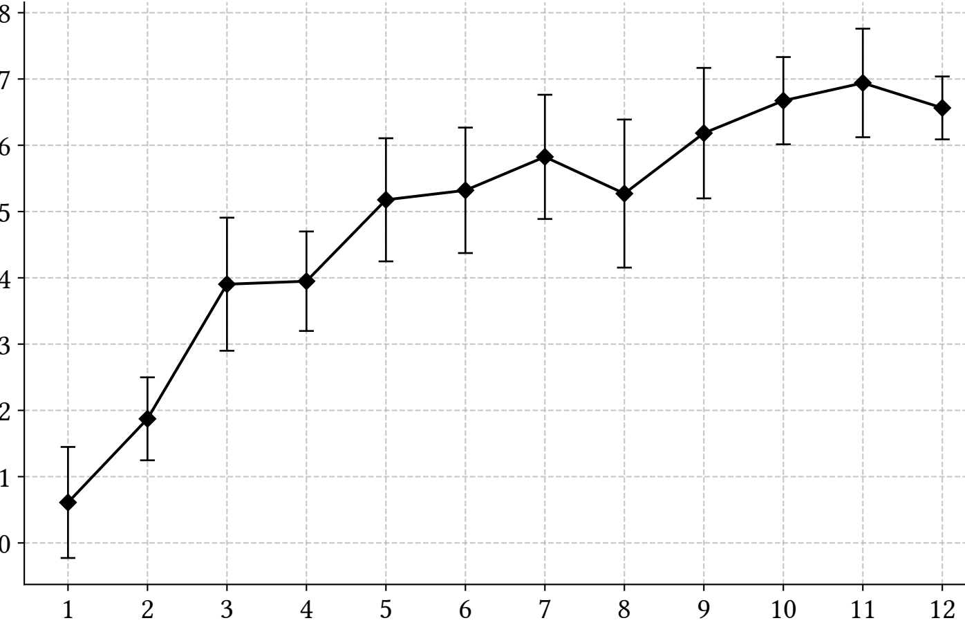
Connected Components
