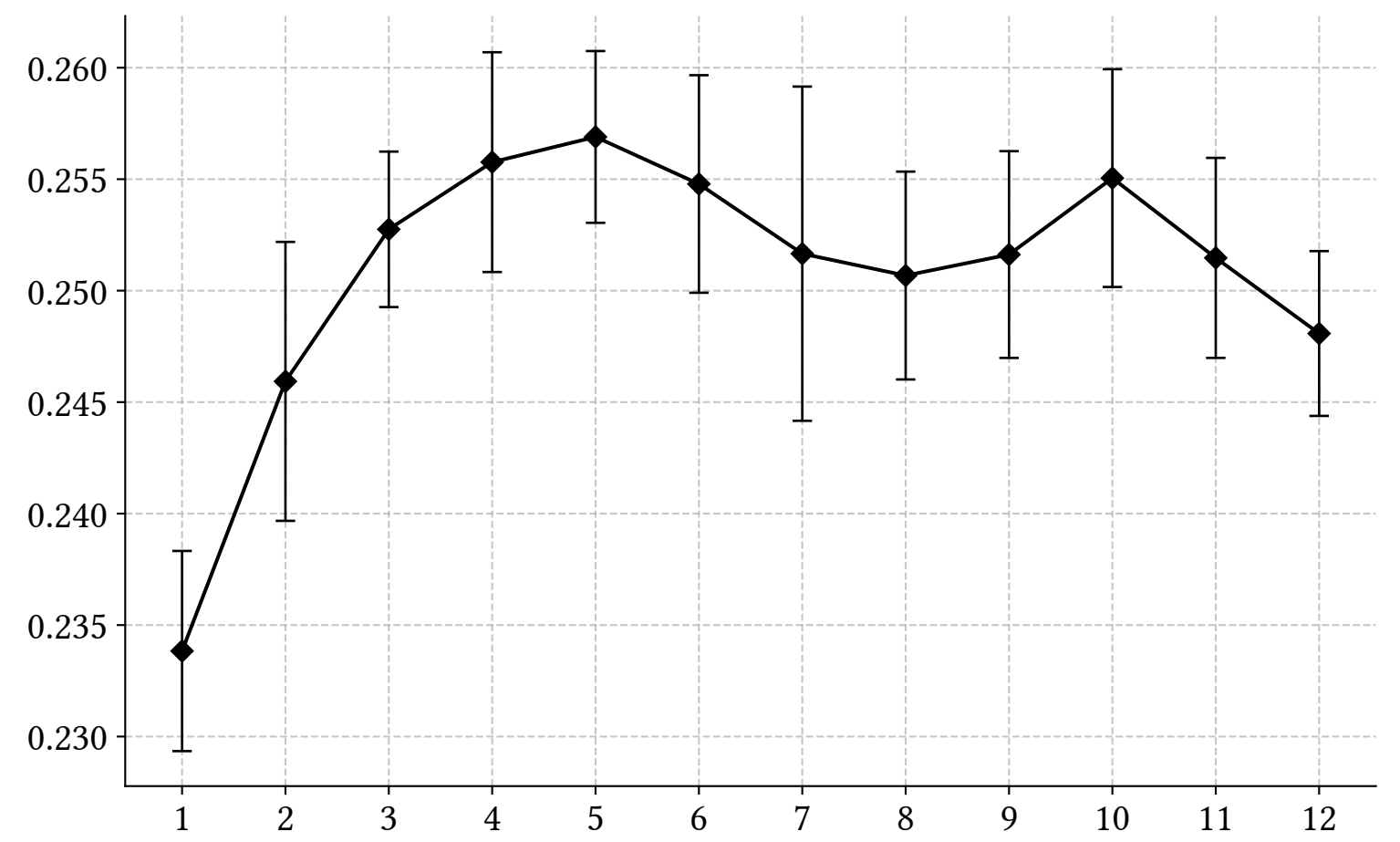
PCP-MAE
