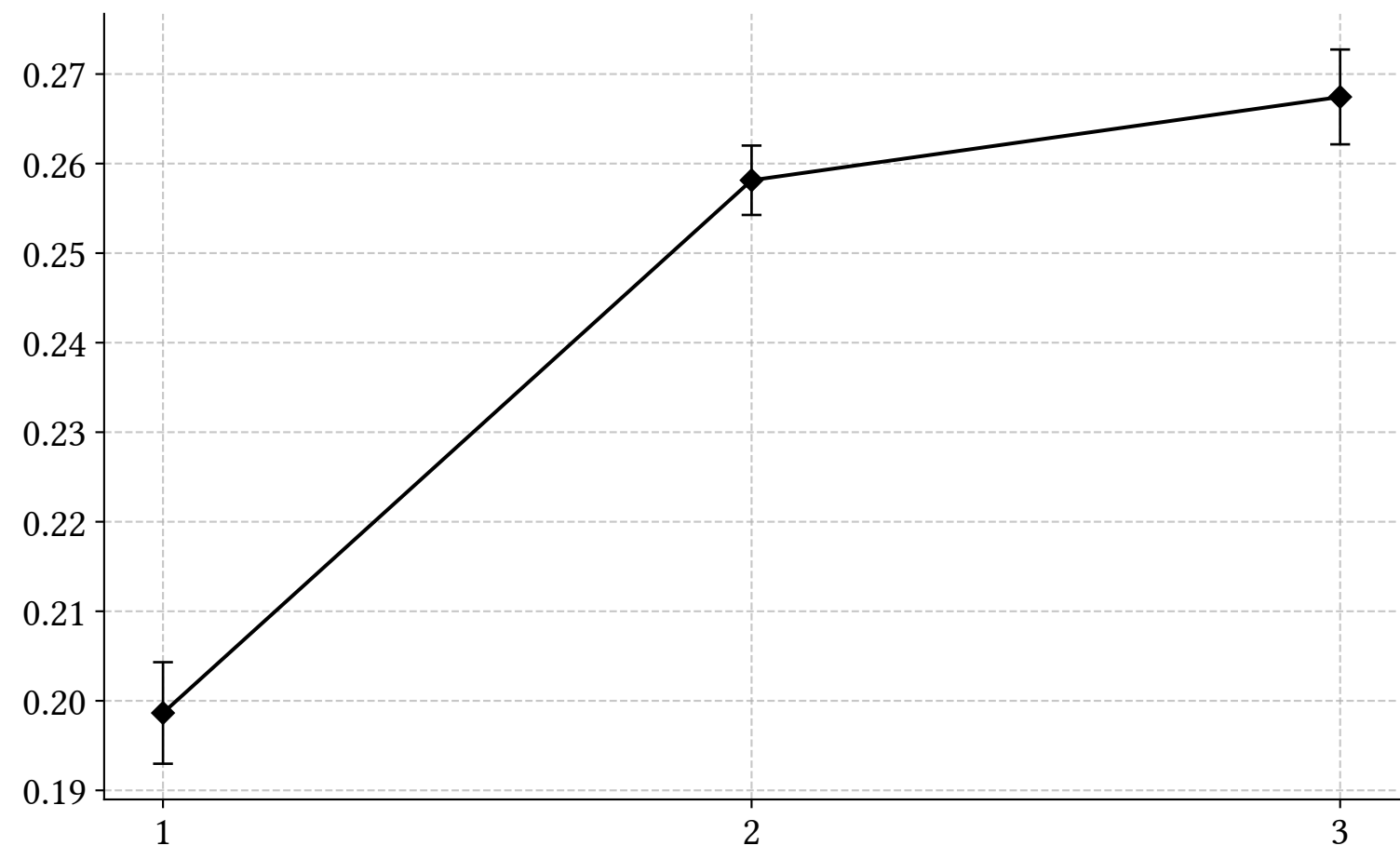
PM2AE
