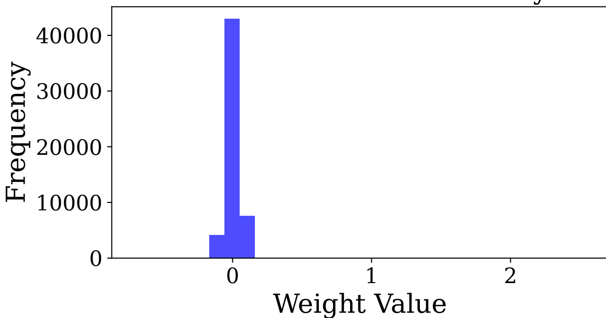
Backdoored Model - Hidden Layer 1
