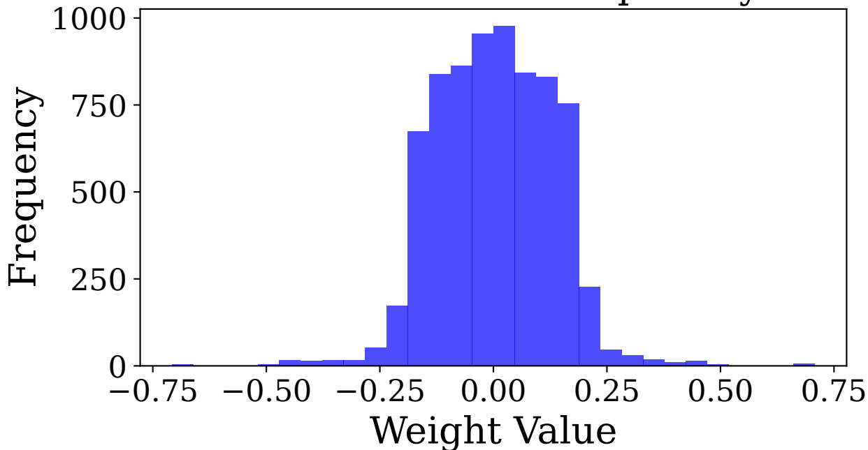
Backdoored Model - Input Layer
