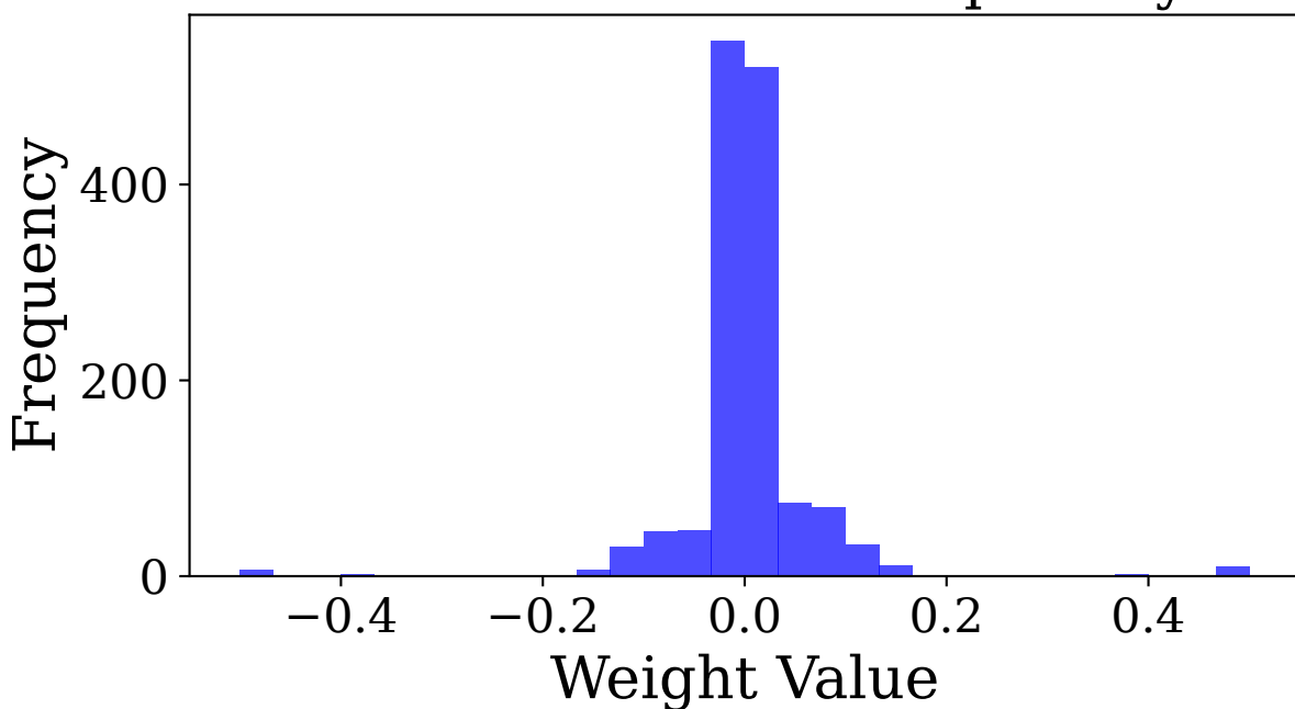
Backdoored Model - Output Layer
