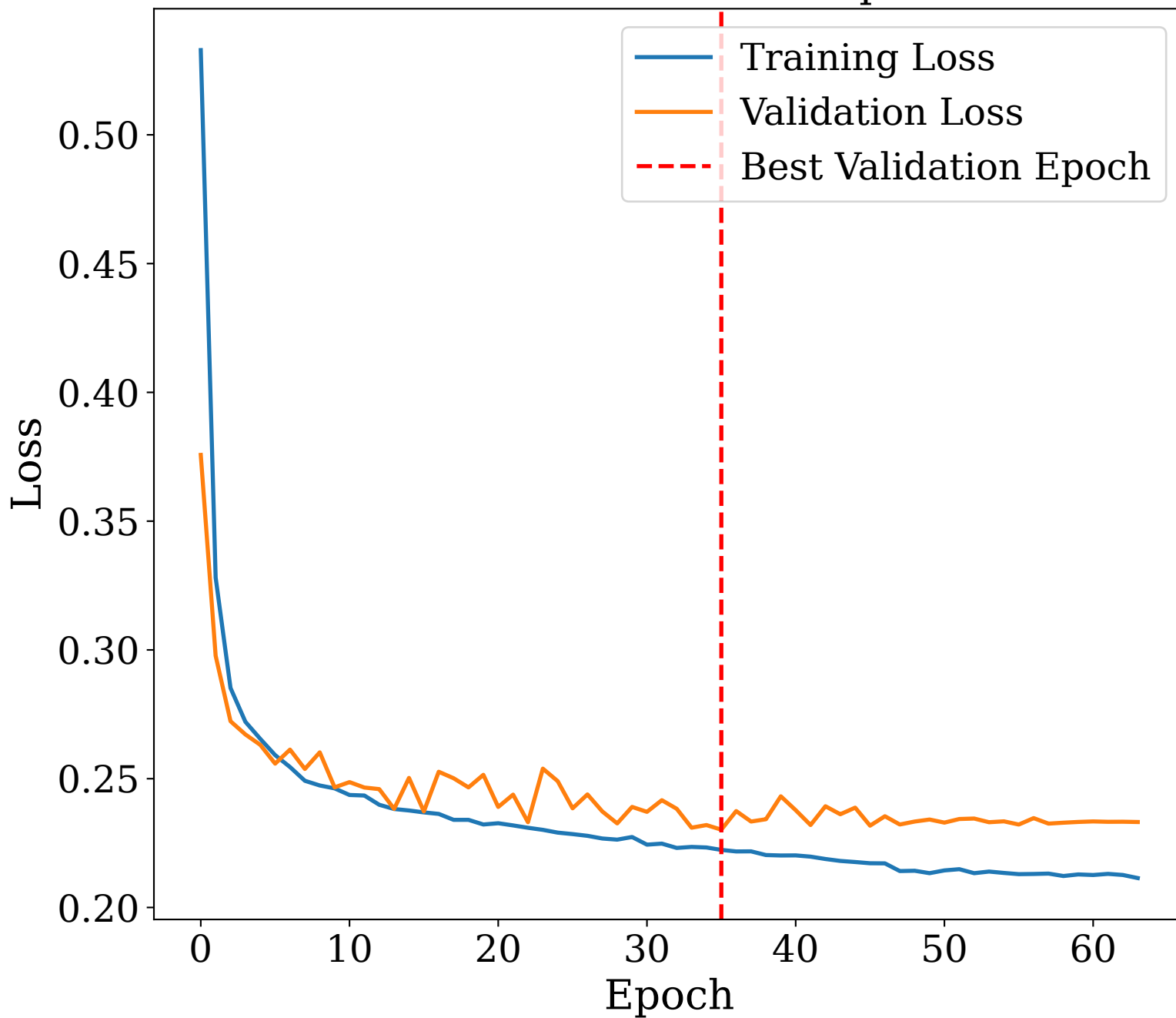
Loan Model Loss over Epochs
