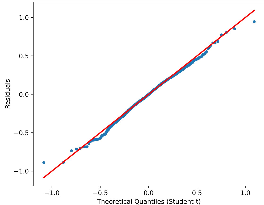
QQ-plot vs Student-t
