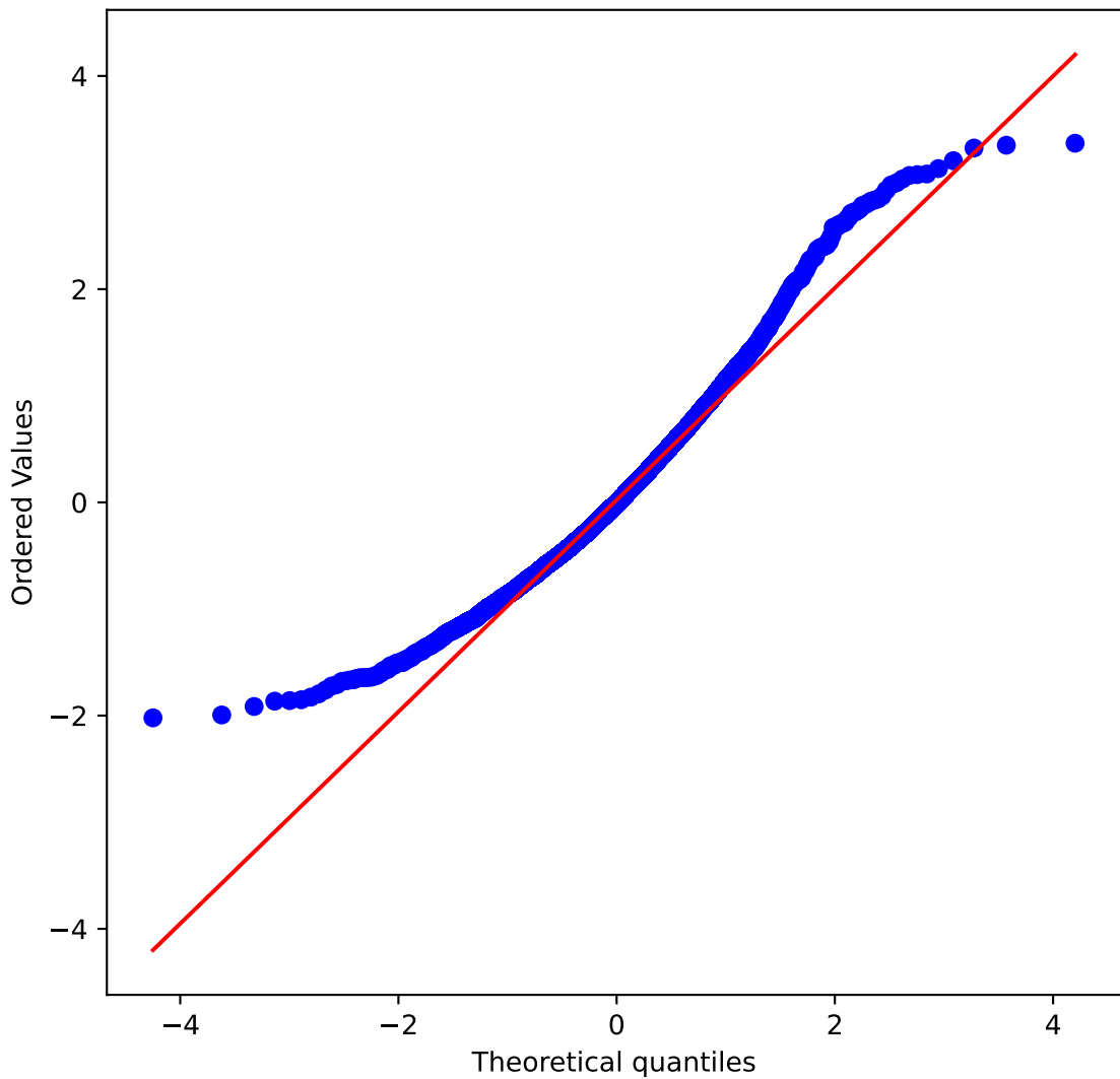
QQ Plot - Student-t
