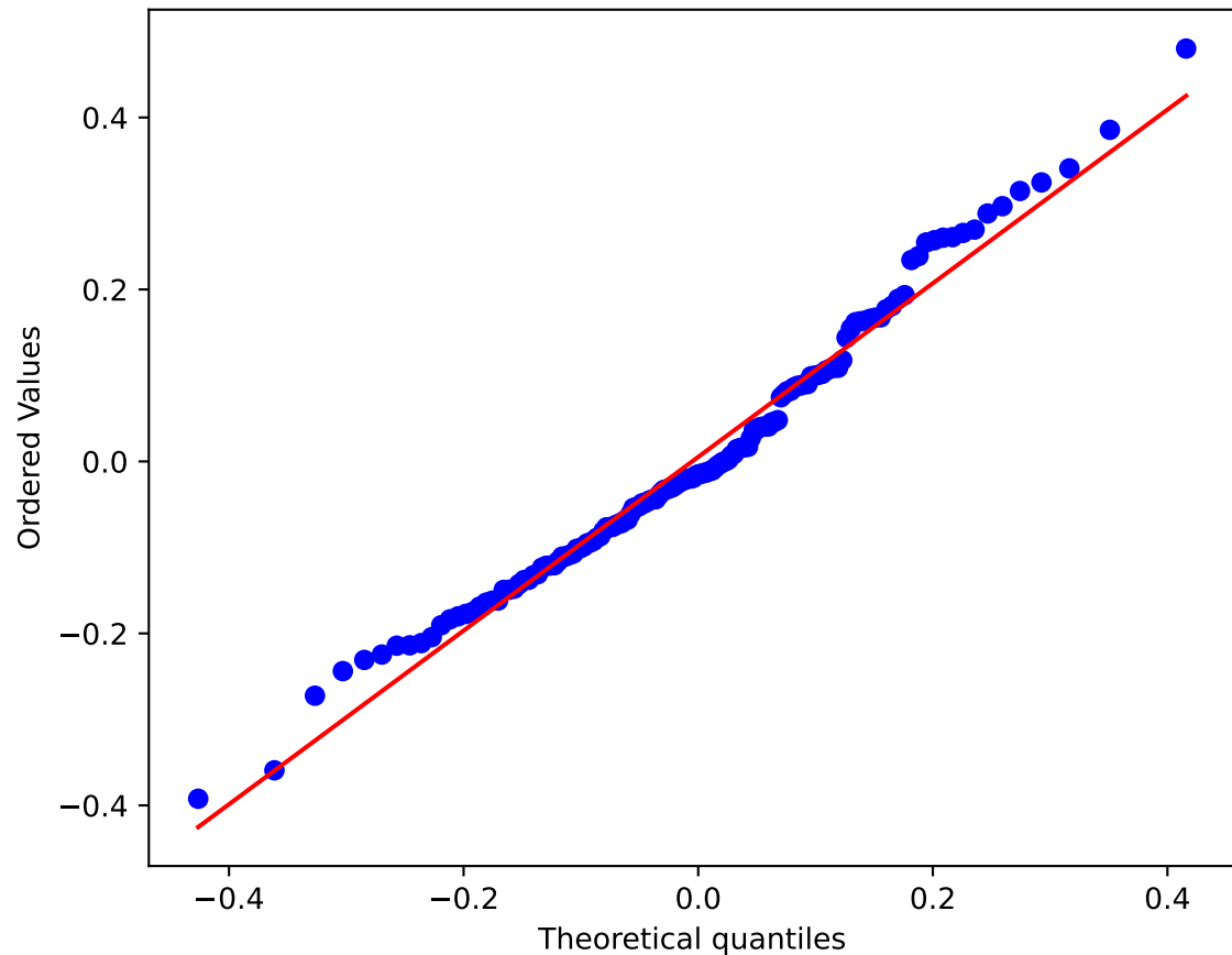
1950 QQ-plot vs Student-t
