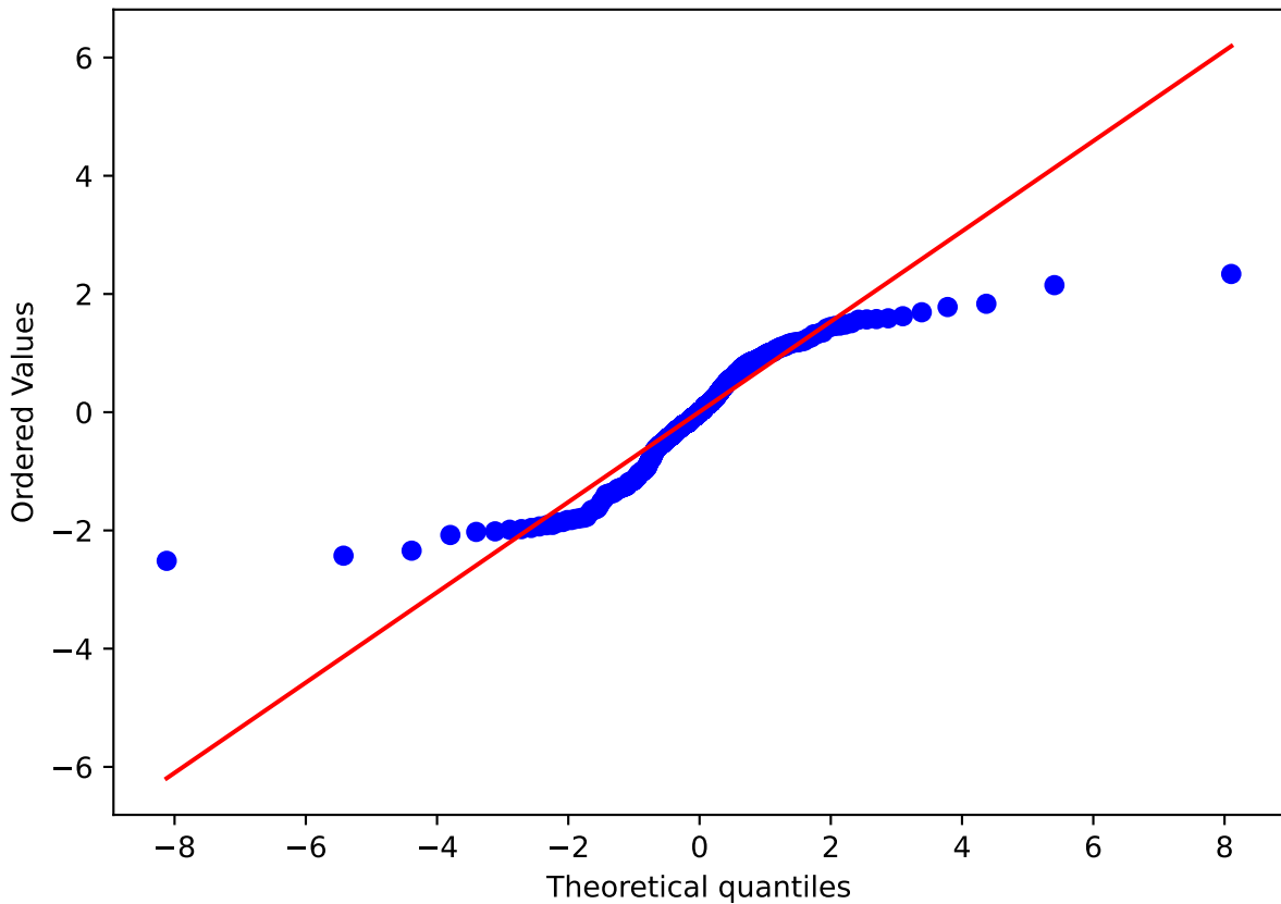
QQ-plot vs Student-t
