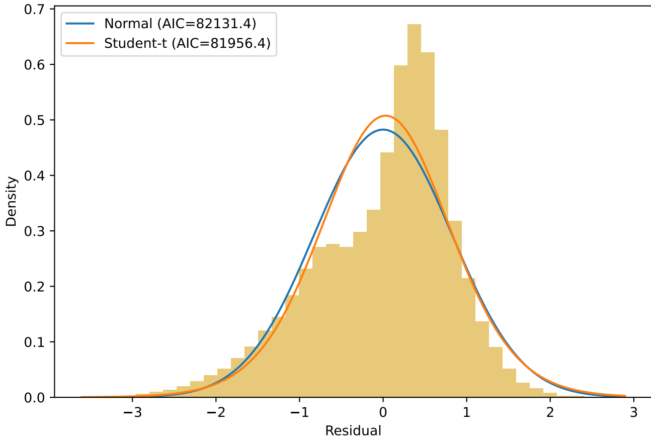
ZIP Codes: Residuals with Normal & Student-t fits
