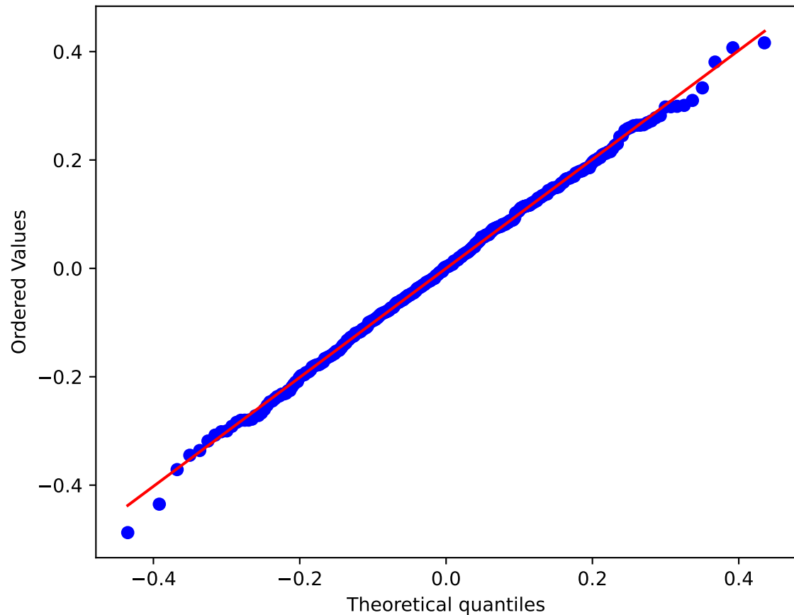
1990 QQ-Plot vs Student-t
