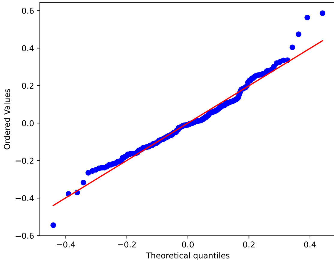
1960 QQ-plot vs Normal
