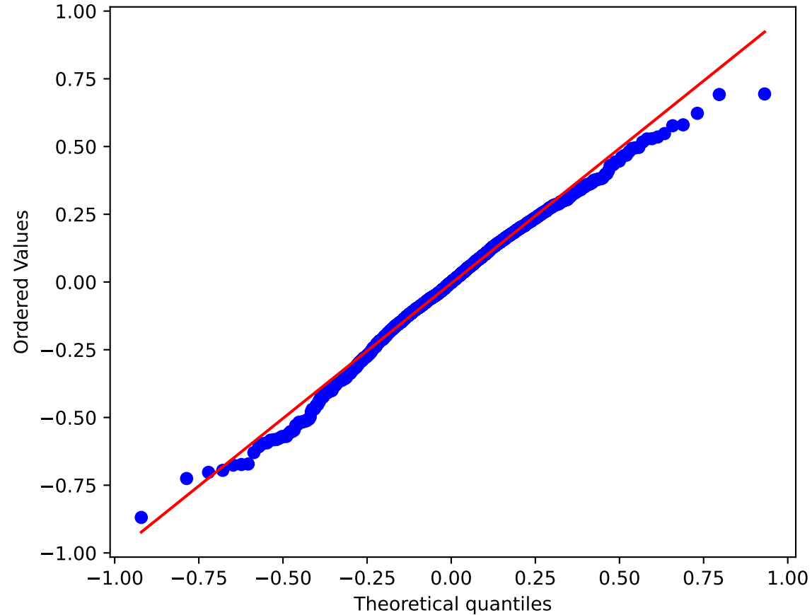
2020 QQ-Plot vs Student-t
