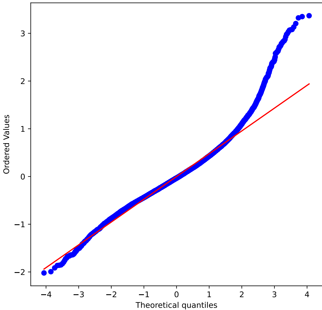
QQ Plot - Normal
