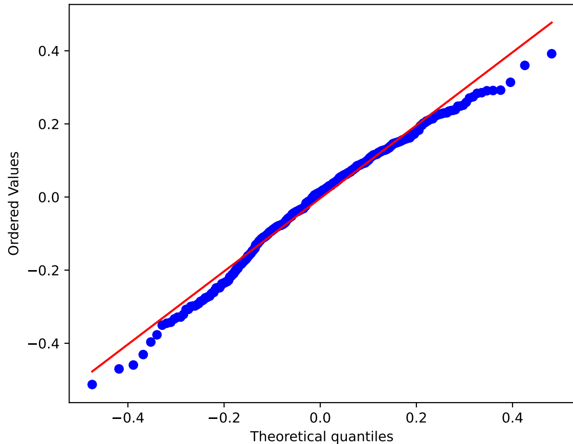
2010 QQ-Plot vs Student-t
