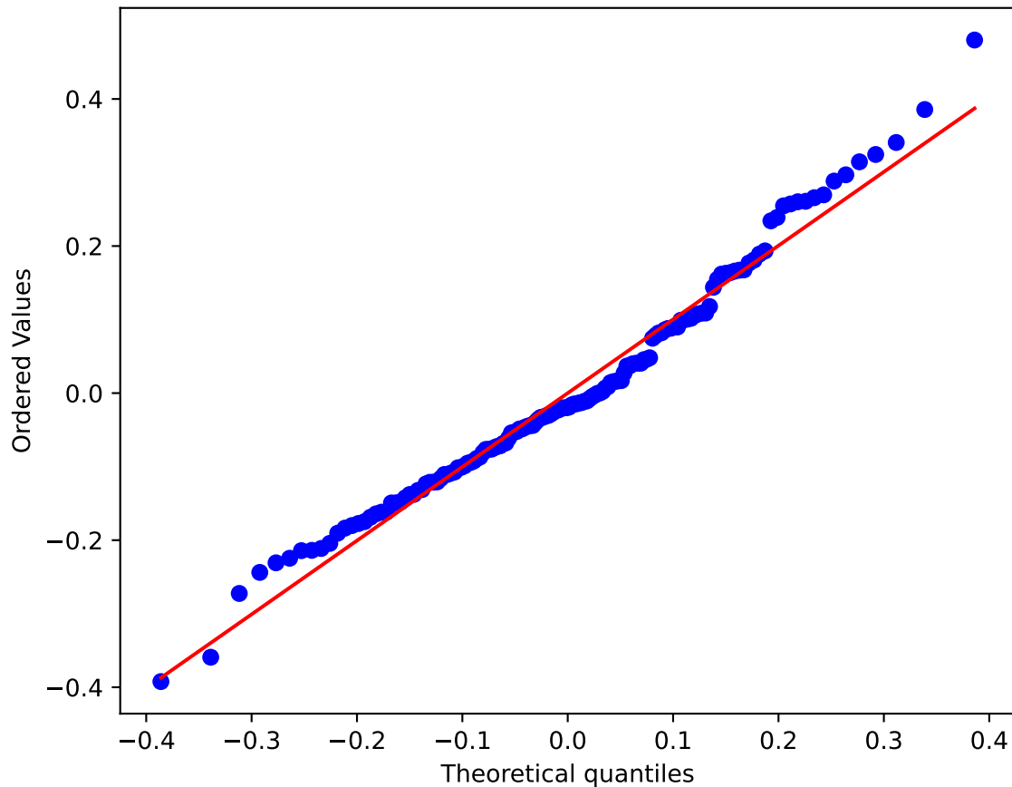
1950 QQ-plot vs Normal
