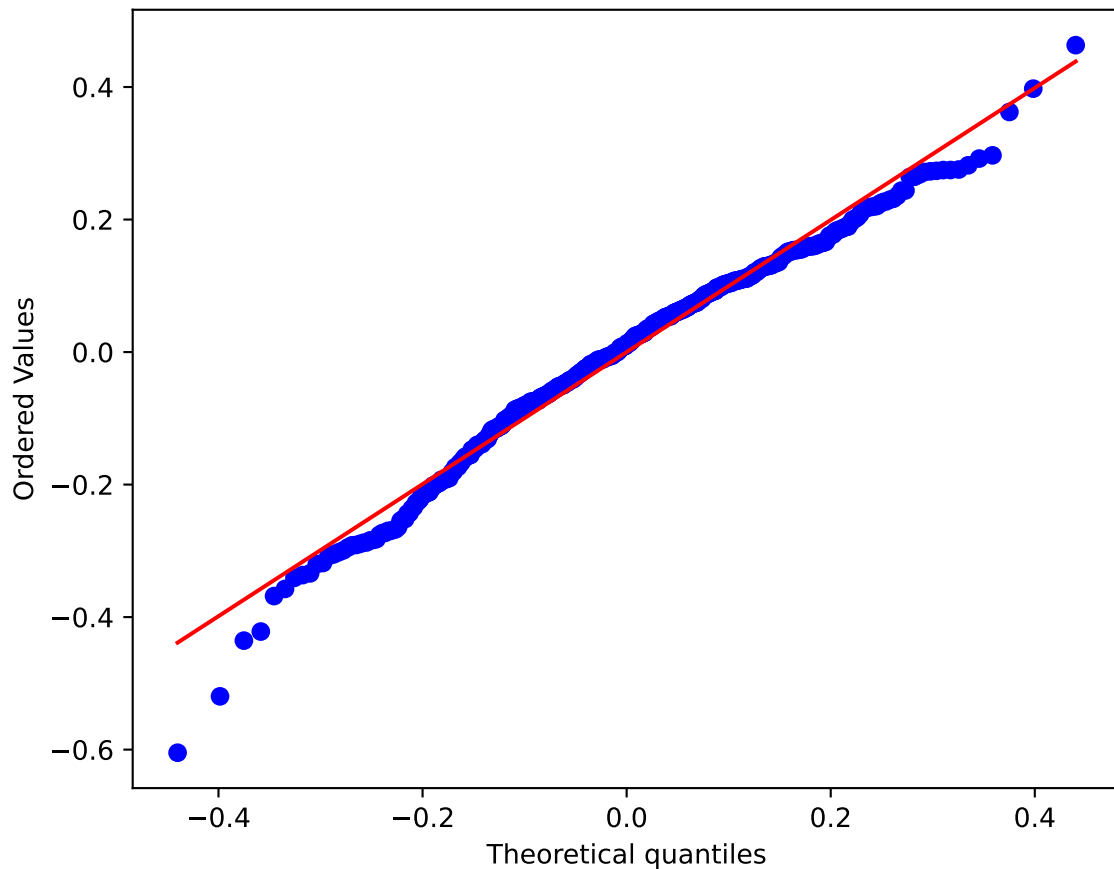
2000 QQ-Plot vs Normal
