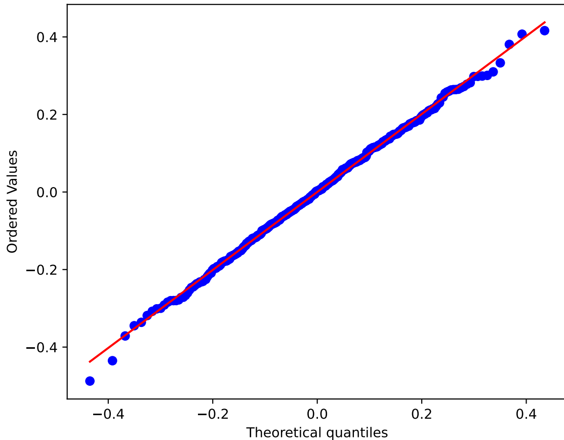
1990 QQ-Plot vs Normal
