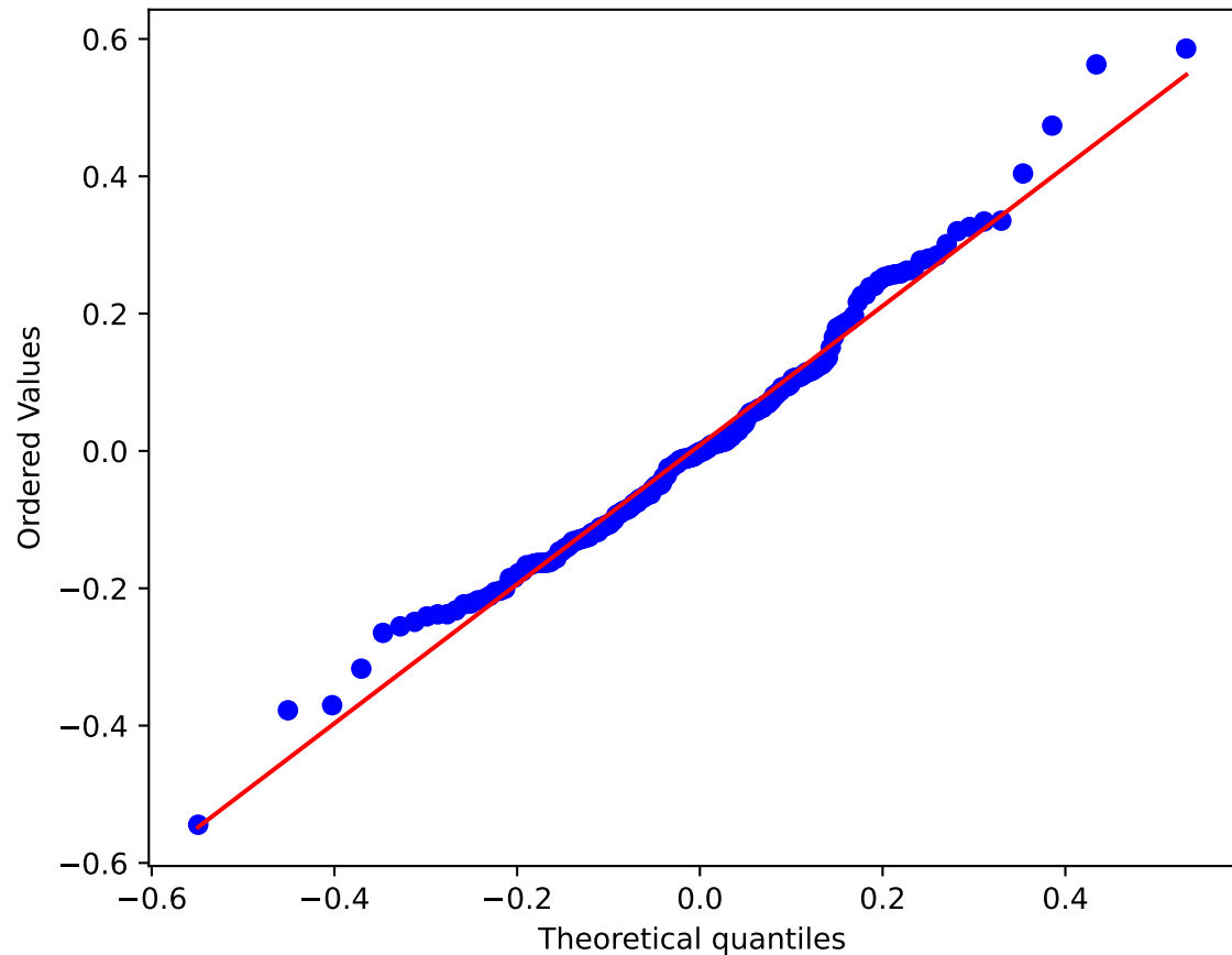
1960 QQ-plot vs Student-t
