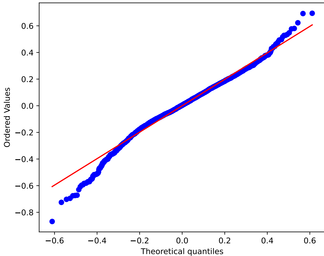
2020 QQ-Plot vs Normal
