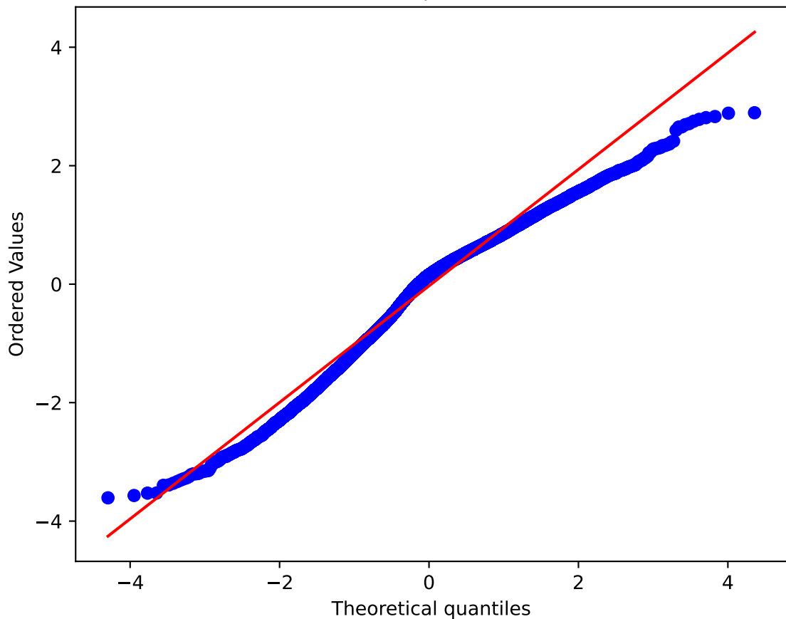
ZIP Codes: QQ-plot vs Student-t
