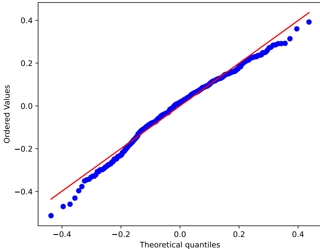
2010 QQ-Plot vs Normal
