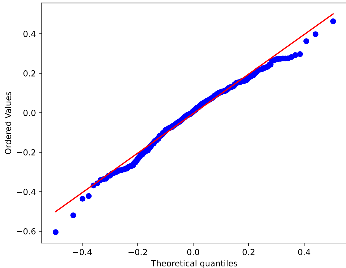
2000 QQ-Plot vs Student-t
