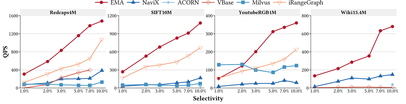
Figure 1: QPS for range+range biased multi-predicate query at 1%-10% selectivity with 95% recall@10.
