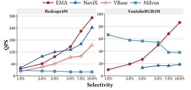
Figure 5: Label-range query at 95% recall@100.
