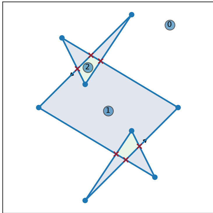
(c) self-intersecting, index two
