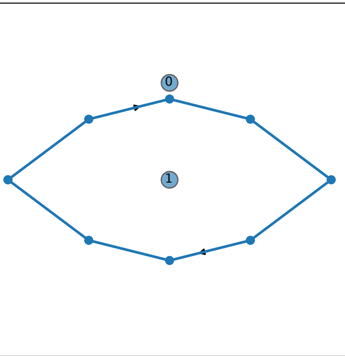
(a) convex, index one
