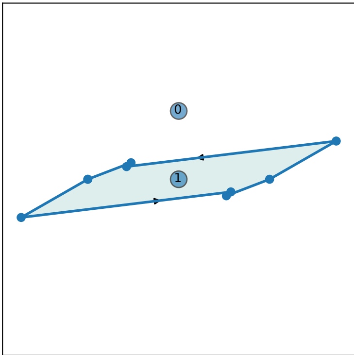
(b) nonconvex, index one
