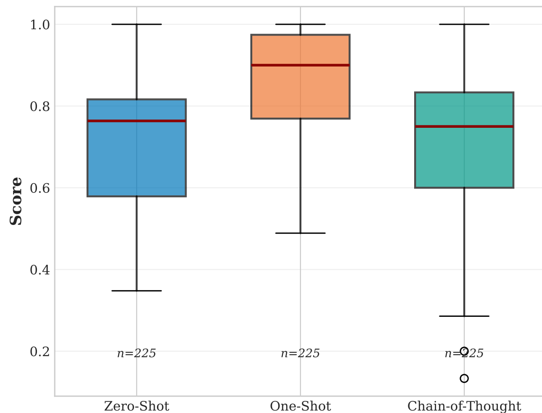
Correctness
