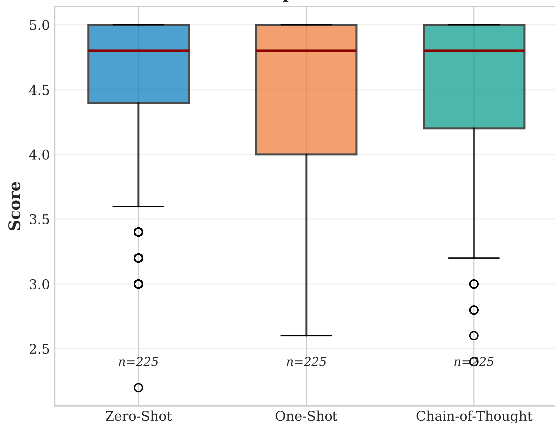
Hallucination
