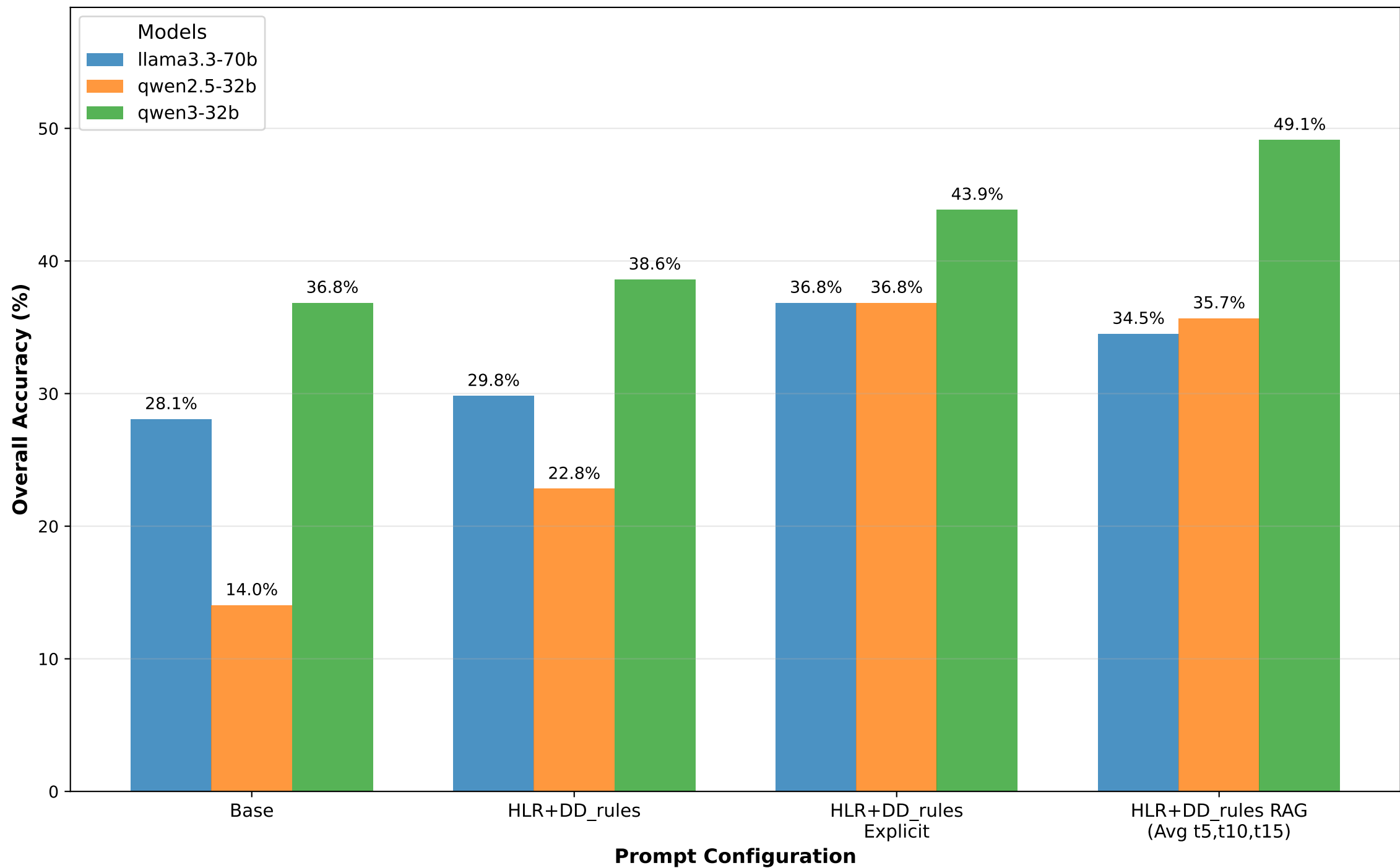
Model Accuracy by Prompt Configurations
