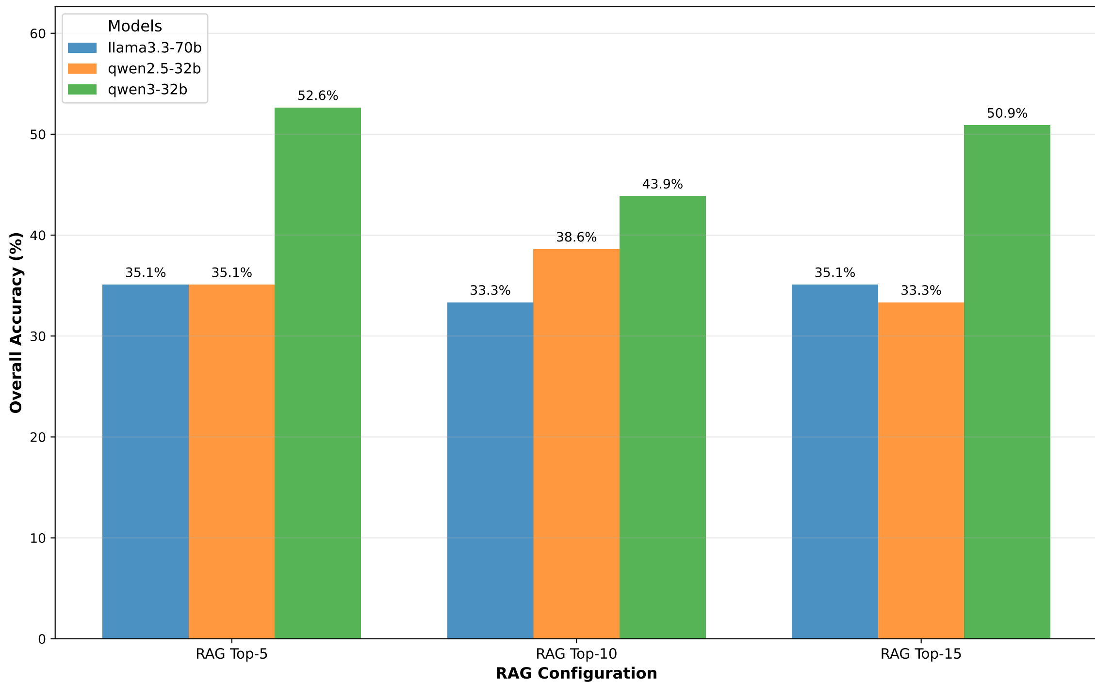
RAG Variants Comparison: HLR+DD_rules with Different Top-K Values
