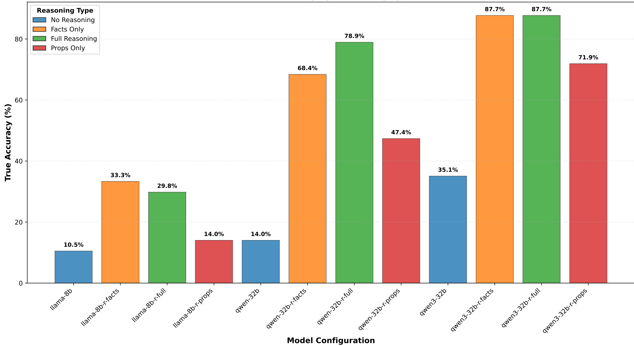
LLM Accuracy by Reasoning Type
