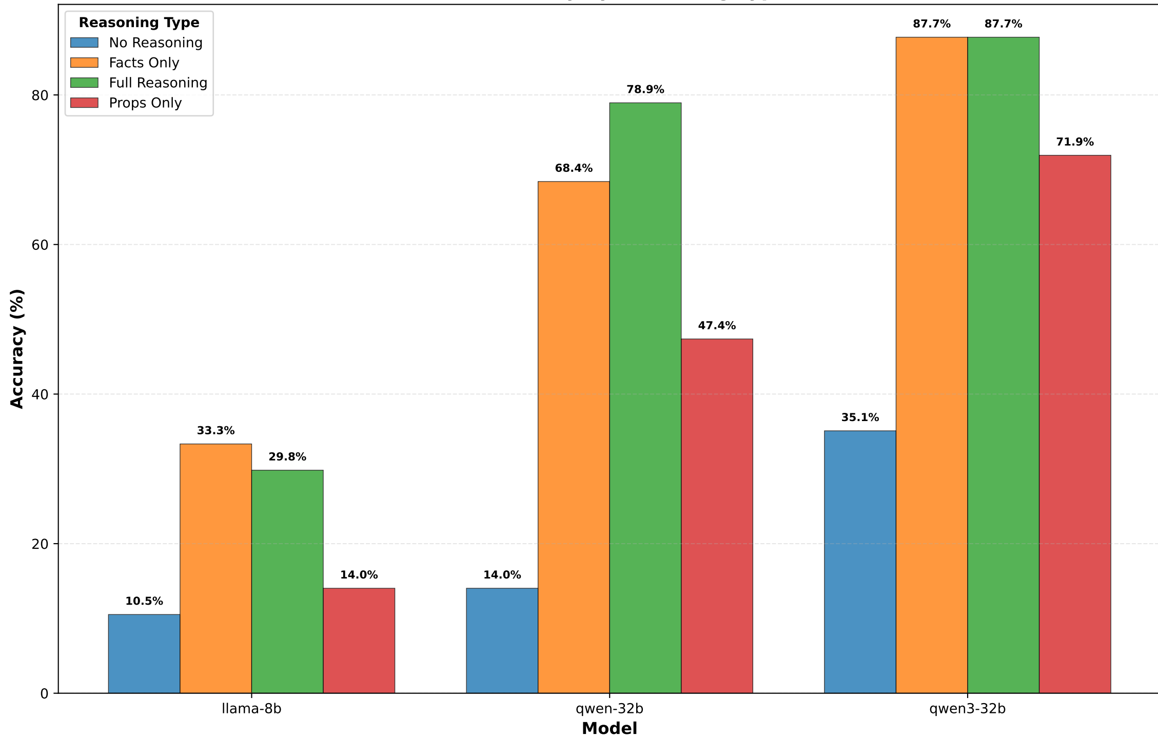
LLM Accuracy by Reasoning Type
