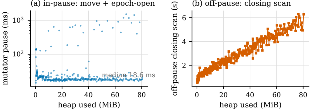
Fig. 4. Sound concurrent revocation (load-side/CLG mode), allocation benchmark growing the heap 0.3 → 82 MiB; 345 cycles, one trace. (a) Mutator pause (relocation + epoch-open), log scale: median 18.6 ms, p90 33 ms across the whole range; the tail (max 1.5 s, ~1 cycle in 10 late in the run) is the epoch-open’s page-table component, which grows with pages touched during the previous closing scan. (b) The heap-linear closing scan (0.6 → 6.3 s) runs on the collector thread with mutators live. For comparison, the synchronous design pays panel (b) inside panel (a)’s pause.
