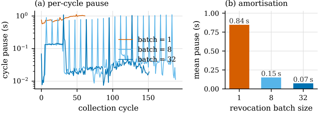
Fig. 3. Batched revocation, IntegrityGC under the concurrent collector. (a) Per-cycle pause, log scale: with batching most cycles pause only for relocation ( \sim 15\text{--}25 ms); the sweep cost concentrates in every N th cycle. (b) Mean pause per cycle falls from 0.84 s to 0.07 s ( 11.9\times ) at batch size 32. The integrity test passes at every batch size.
