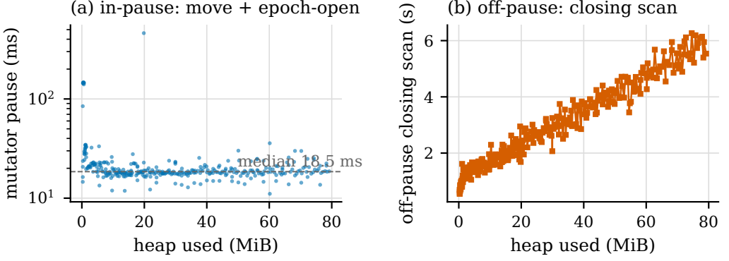
Fig. 4. Sound concurrent revocation (load-side/CLG mode), allocation benchmark growing the heap 0.3 → 79 MiB; one trace, all 334 cycles shown, no filtering. (a) Mutator pause (relocation + epoch-open), log scale: median 18.5 ms, p90 25.7 ms, p99 146.5 ms, max 461 ms (the largest pauses sit in the early class-loading phase; the final 100 cycles, at the largest heap, have p90 24.3 ms and none over 100 ms). (b) The heap-linear closing scan (0.70 → 5.54 s) runs on the collector thread with mutators live. The synchronous design pays panel (b) inside panel (a)’s pause.
