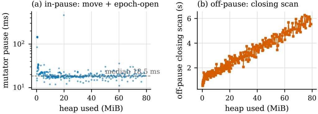
Fig. 4. Sound concurrent revocation (load-side/CLG mode), allocation benchmark growing the heap 0.3 → 79 MiB; one trace, all 334 cycles shown, no filtering. (a) Mutator pause (relocation + epoch-open), log scale: median 18.5 ms, p90 25.7 ms, p99 146.5 ms, max 461 ms (the largest pauses sit in the early class-loading phase; the final 100 cycles, at the largest heap, have p90 24.3 ms and none over 100 ms). (b) The heap-linear closing scan (0.70 → 5.54 s) runs on the collector thread with mutators live. The synchronous design pays panel (b) inside panel (a)’s pause.
