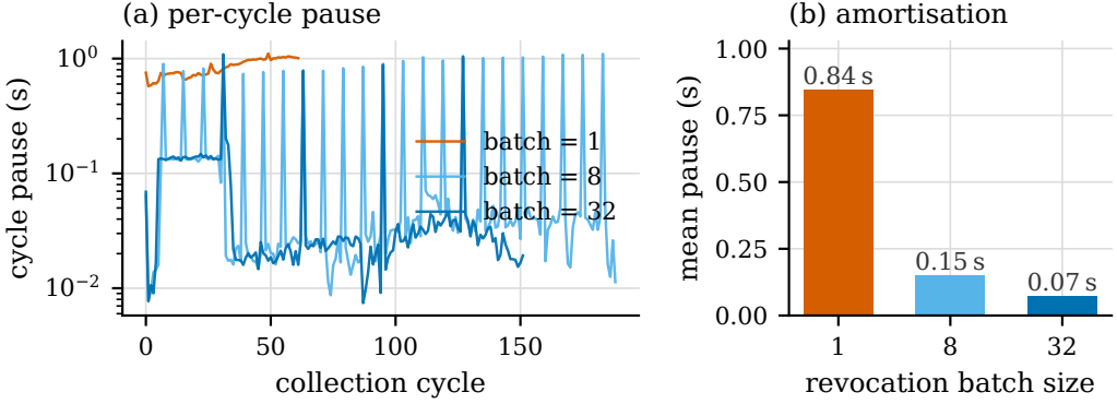
Fig. 3. Batched revocation, IntegrityGC under the concurrent collector. (a) Per-cycle pause, log scale: with batching most cycles pause only for relocation ( \sim 15\text{--}25\text{ ms} ); the sweep cost concentrates in every N th cycle. (b) Mean pause per cycle falls from 0.84\text{ s} to 0.07\text{ s} ( 11.9\times ) at batch size 32. (Data from runs that completed; batch > 1 is not a sound configuration—see text.)
