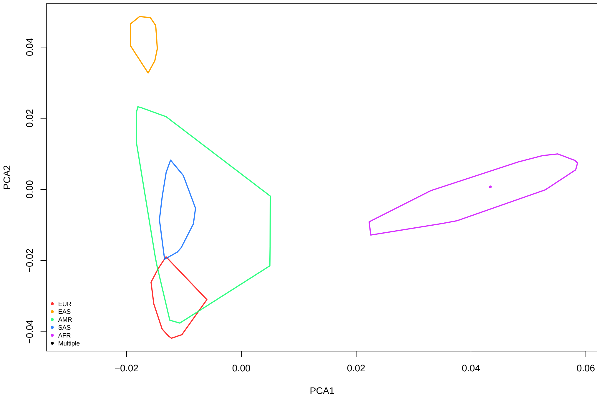
Target samples with reference populations (#SNPs=17437)
