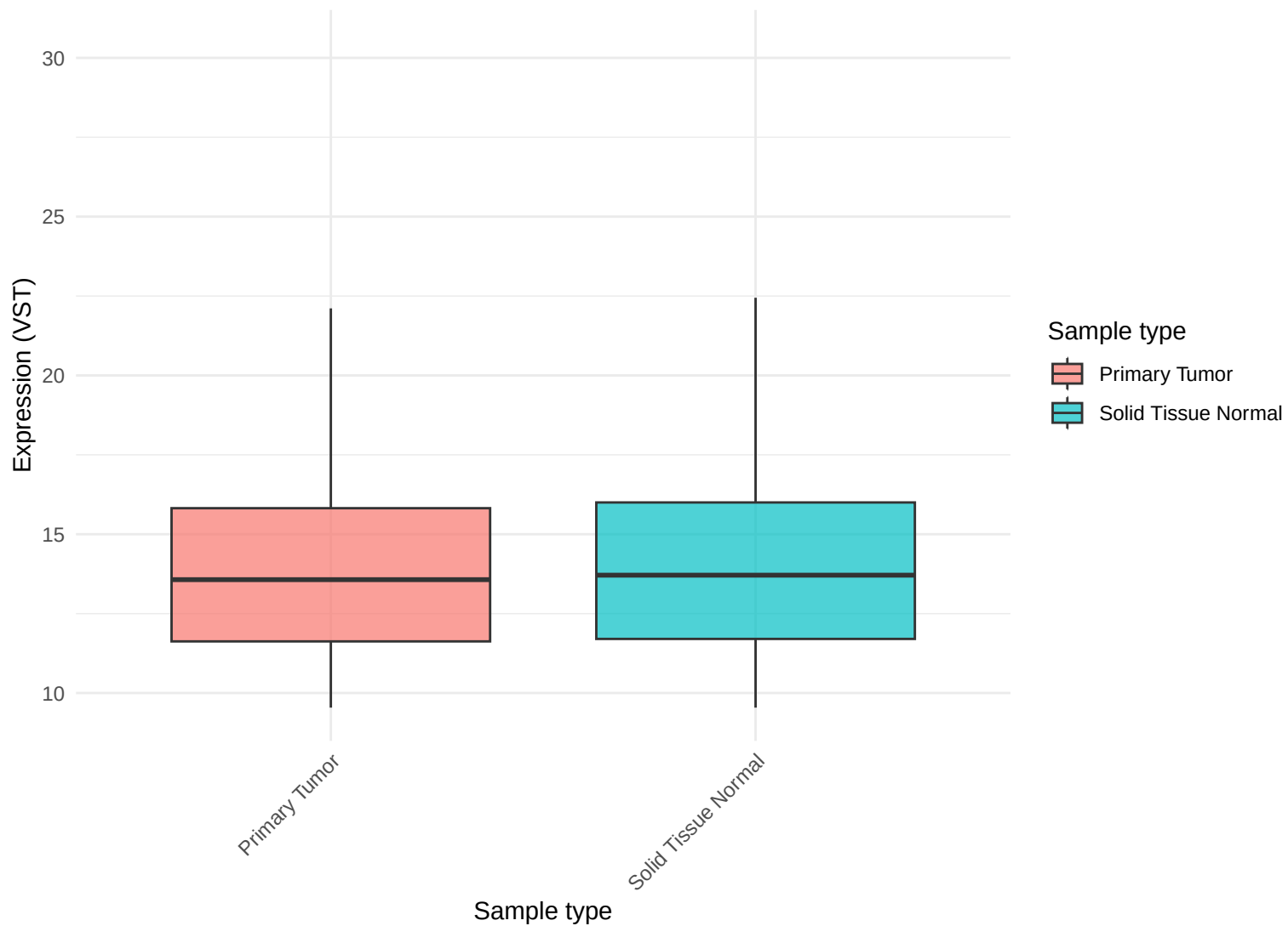
Subset VST expression distribution by sample type
