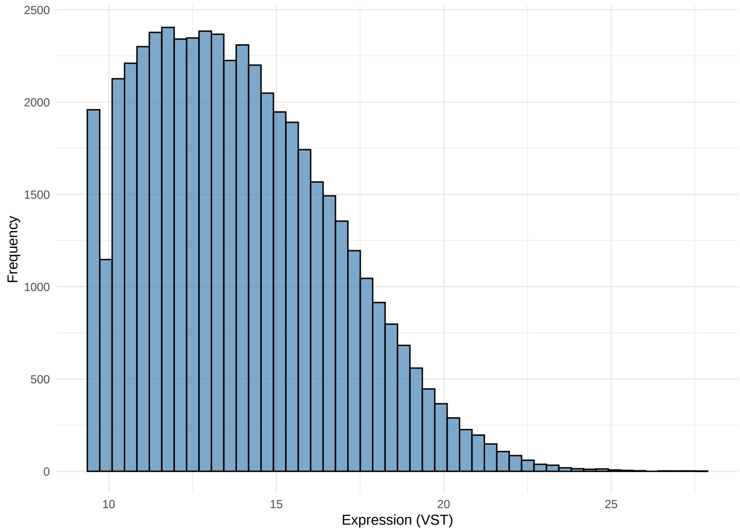
Histogram of subset VST expression values
