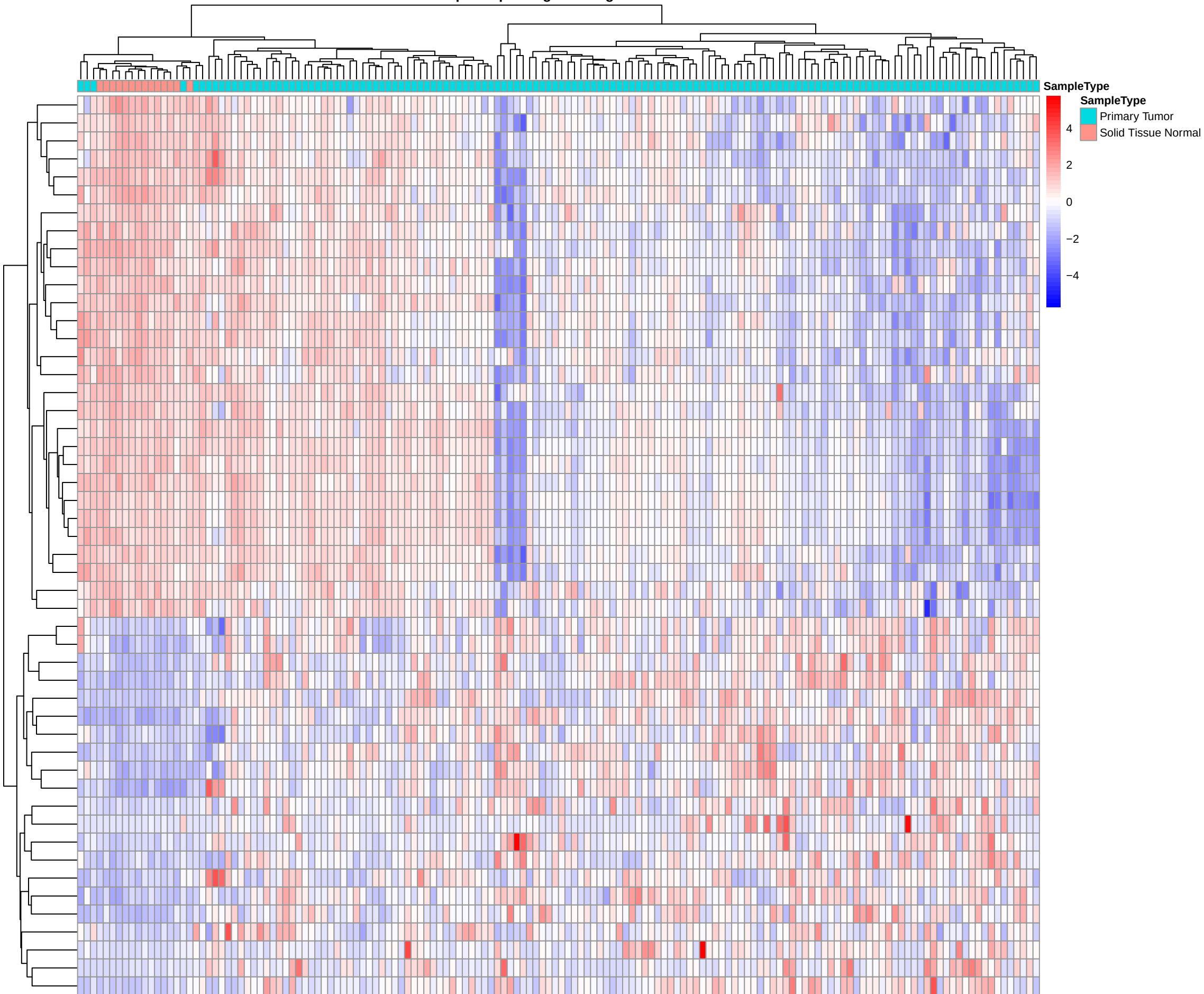
Heatmap of top 50 significant genes in subset
