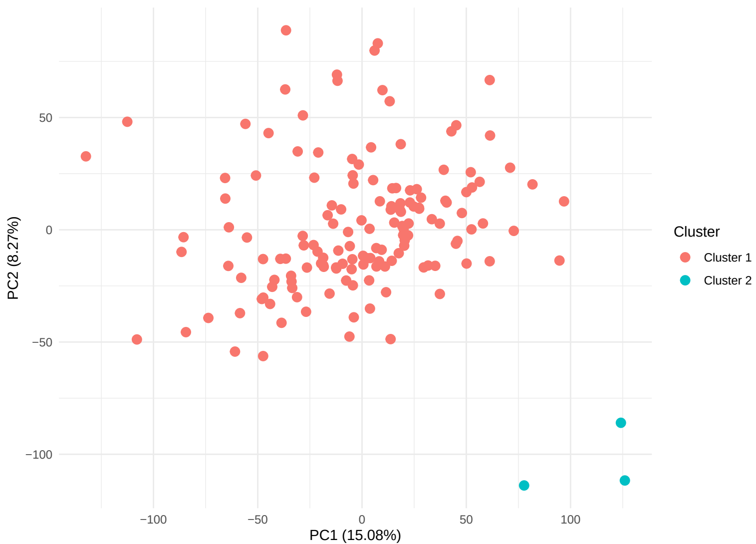
PCA of TCGA-PRAD Samples with Hierarchical Clustering
