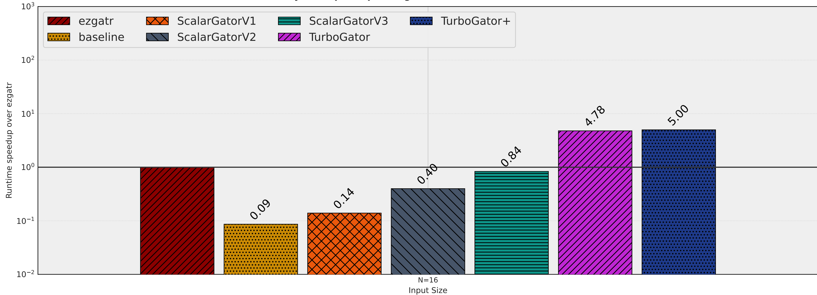
Runtime (cycles) speedup vs ezgatr - Intel Core 7 240H (P-core, 2.5GHz)
