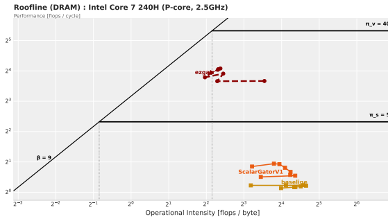
Fig. 8: DRAM roofline, high op-count versions.
