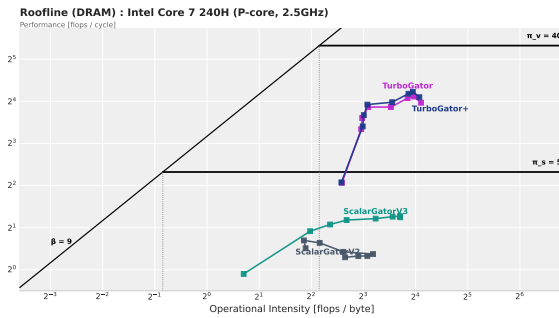
Fig. 9: DRAM roofline, low op-count versions.
