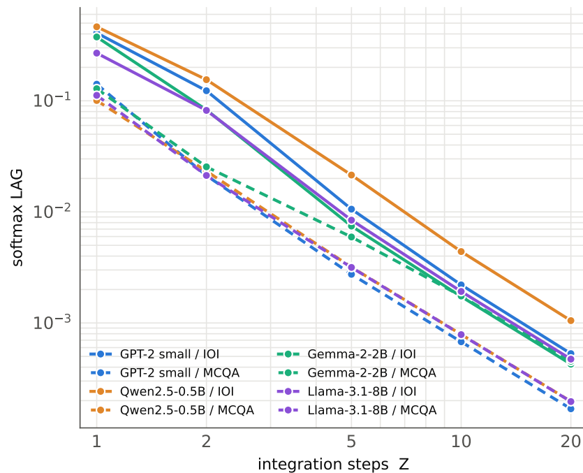
(c) softmax: Z-step IG (solid/dashed/dotted = IOI/MCQA)
