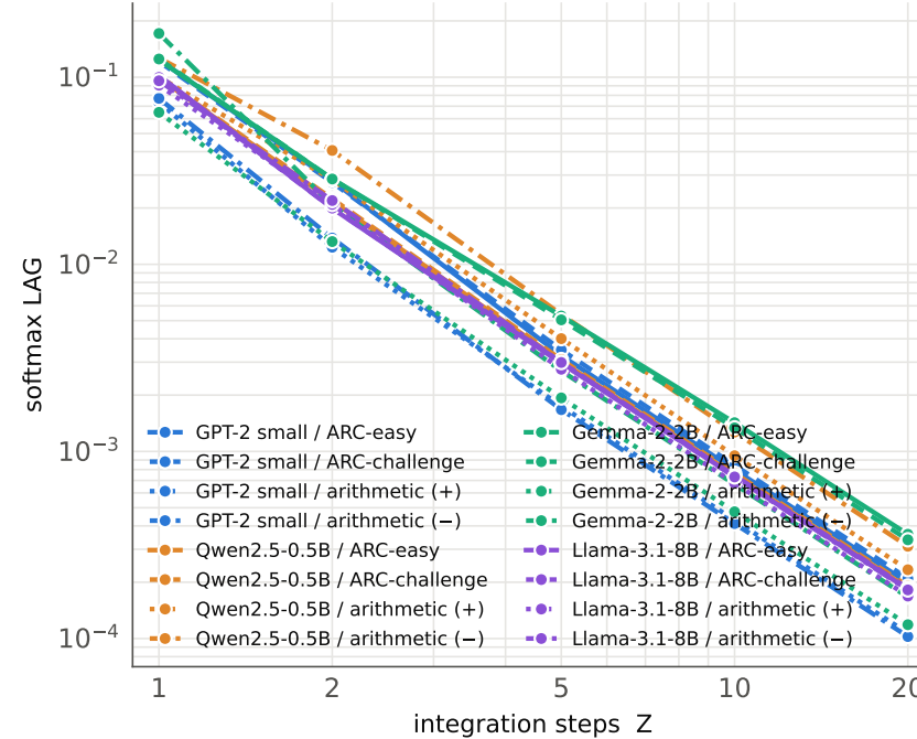
(e) softmax: Z-step IG residual (line style = task, see legend)
