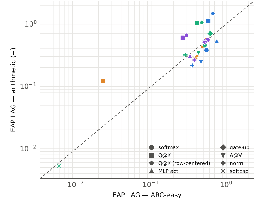
(f) task effect: same op, arithmetic (−) vs ARC-easy (marker = op, color = model)
